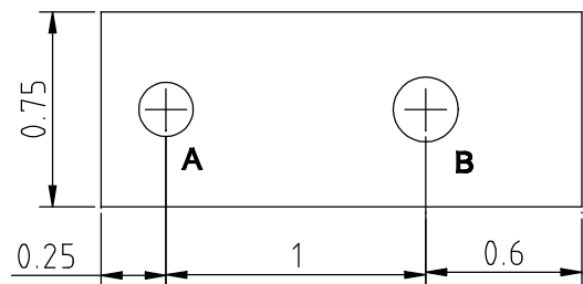
ITEM #3 LEAF MATERIAL=COPPER 0.04 THK HOLE 'A'=0.209 HOLE 'B'=0.25 QTY=72
