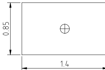
ITEM #4 INSULATION MATERIAL=KAPTON 0.002 THK HOLE=0.15 QTY=64
