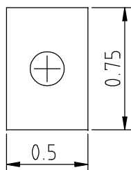
ITEM #2 SPACER MATERIAL=COPPER 0.04 THK HOLE=0.209 QTY=68
