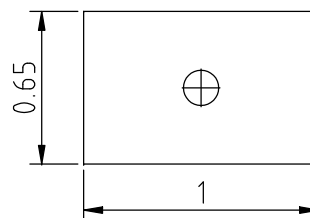
ITEM #5 PLATE MATERIAL=304 S.S 0.062 THK HOLE=0.15 QTY=16
