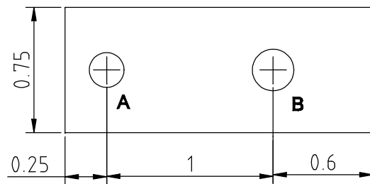
ITEM #3 LEAF MATERIAL=COPPER 0.04 THK HOLE 'A'=0.209 HOLE 'B'=0.25 QTY=296
