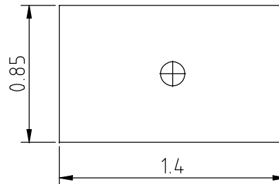
ITEM #4 INSULATION MATERIAL=KAPTON 0.002 THK HOLE=0.15 QTY=280
