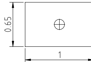
ITEM #5 PLATE MATERIAL=304 S.S 0.062 THK HOLE=0.15 QTY=32
