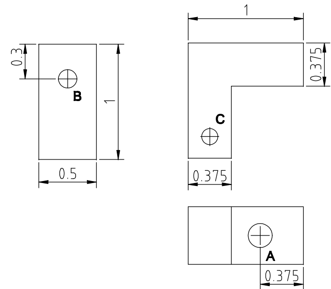
ITEM #9 TERMINAL MATERIAL= COPPER 1/2" X 1" X 1" HOLE 'A' = 0.209 THRU HOLE 'B' = TAP 6-32 X 0.5 DEEP HOLE 'C' = TAP 6-32 THRU QTY=8
