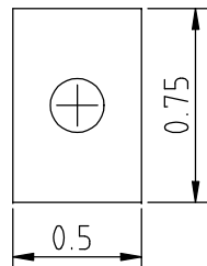
ITEM #1 BASE MATERIAL=COPPER 1/4 X 1/2 X 3/4 HOLE=0.209 QTY=16
