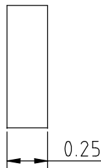
ITEM #1 BASE MATERIAL=COPPER 1/4 X 1/2 X 3/4 HOLE=0.209 QTY=16
