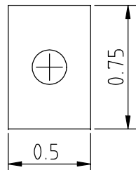
ITEM #2 SPACER MATERIAL=COPPER 0.04 THK HOLE=0.209 QTY=156
