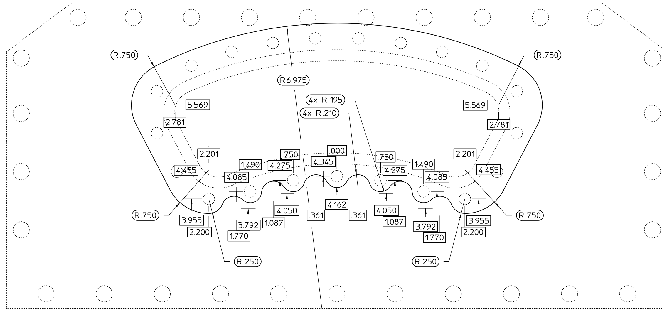
FLANGE INFORMATION
