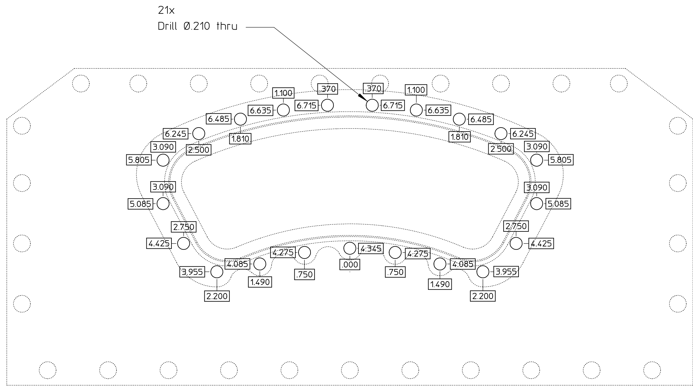
HOLE INFORMATION
