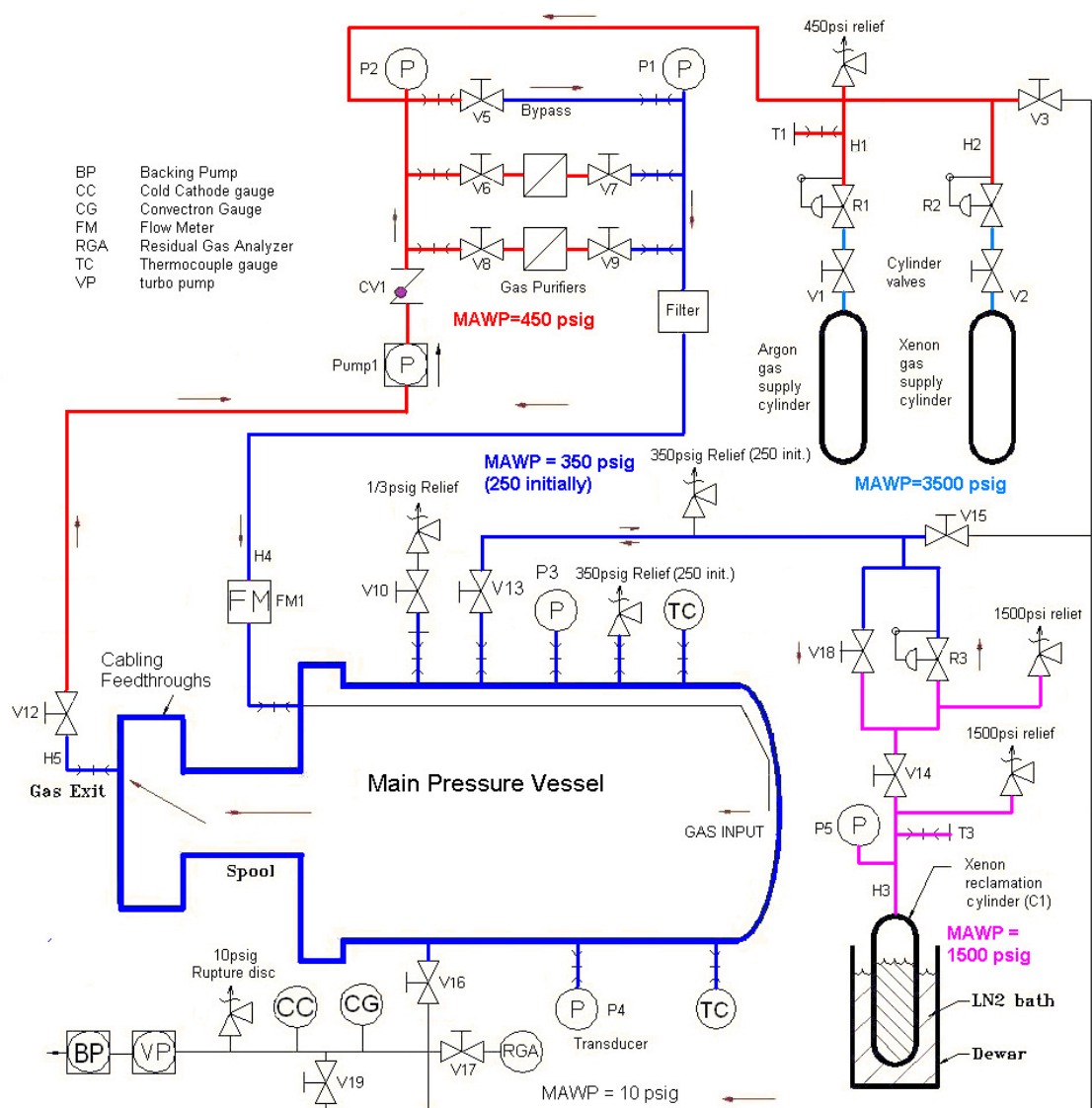
Fig. 5 Gas System Schematic
