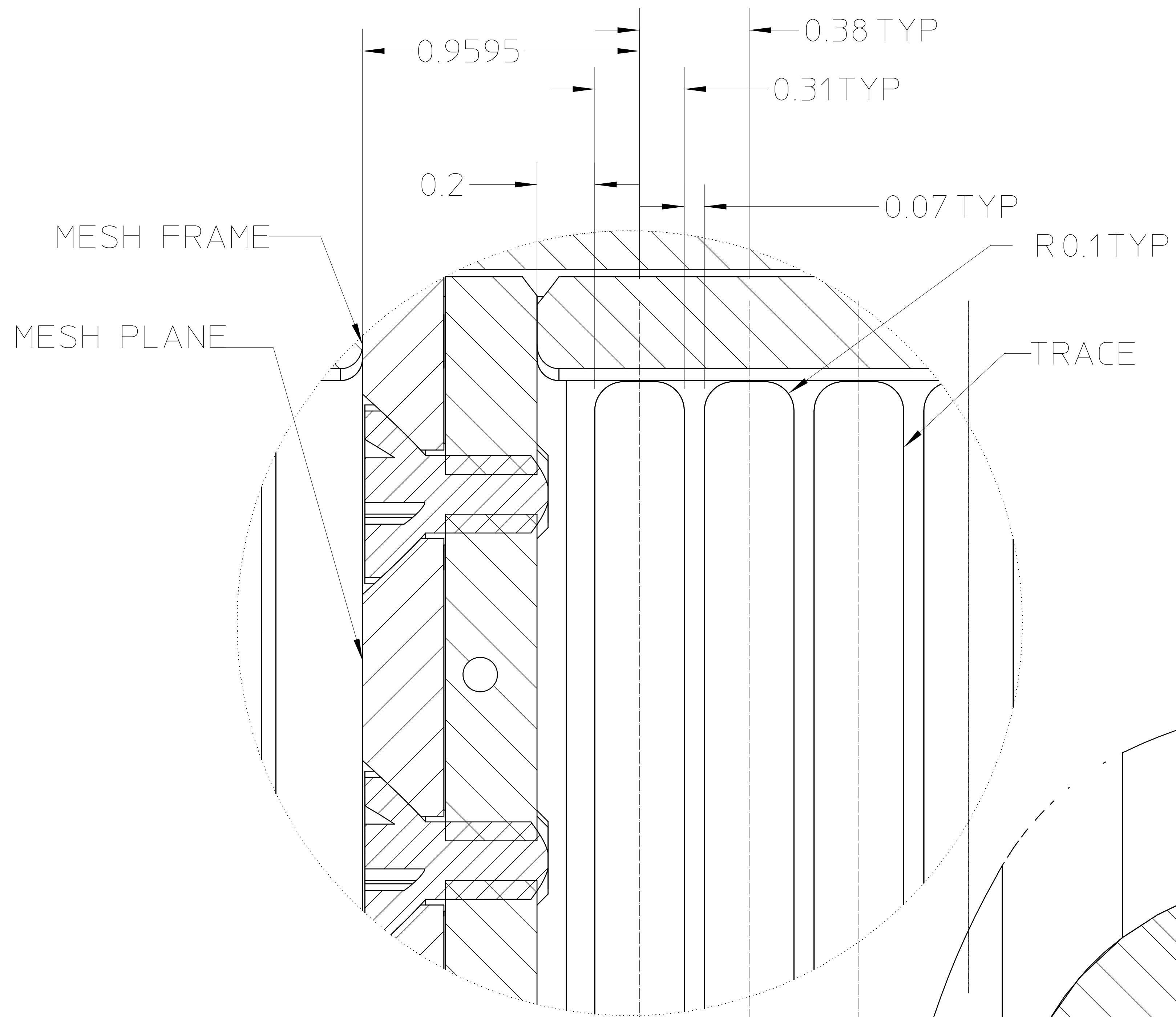
Detail3 SCALE 5:1
