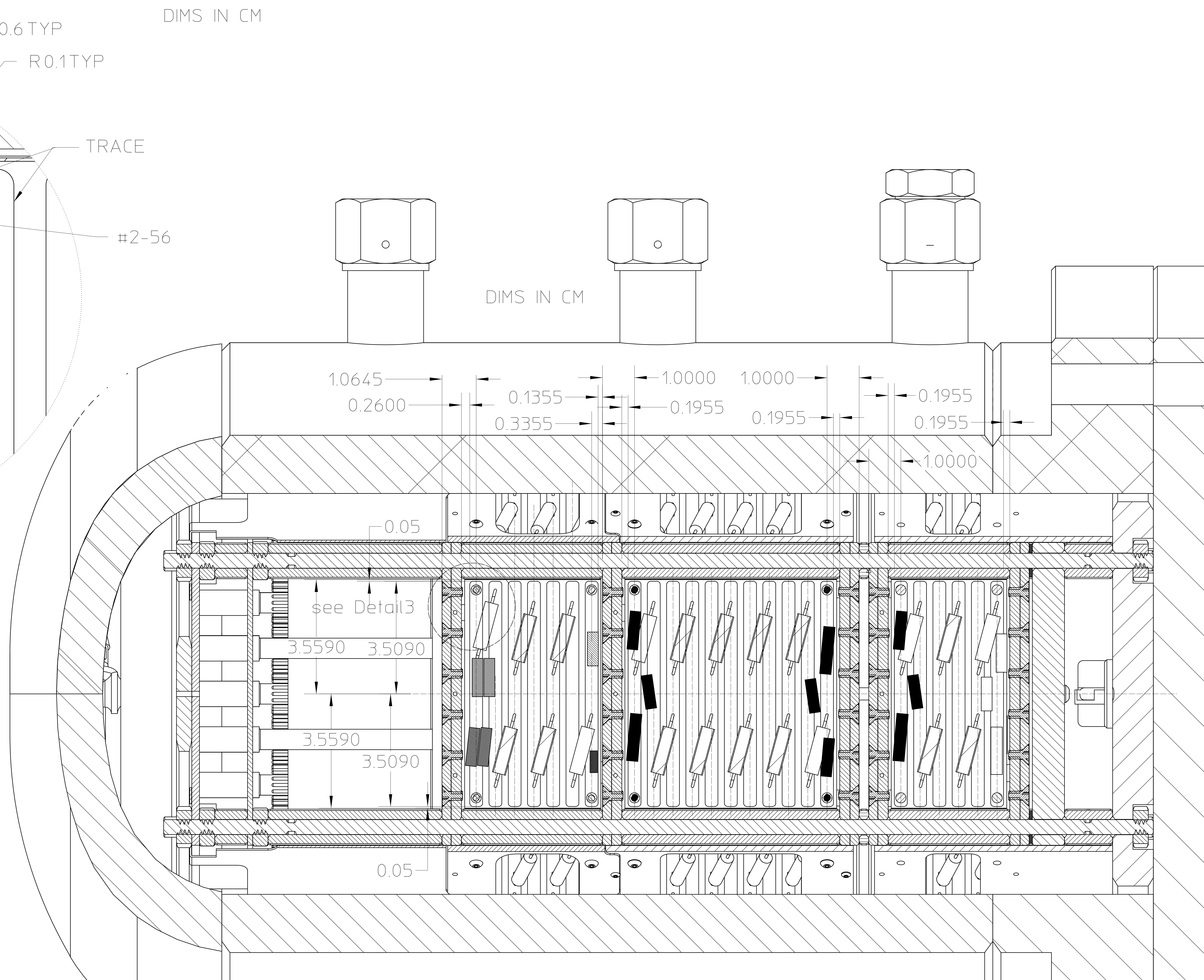
Section F-F
