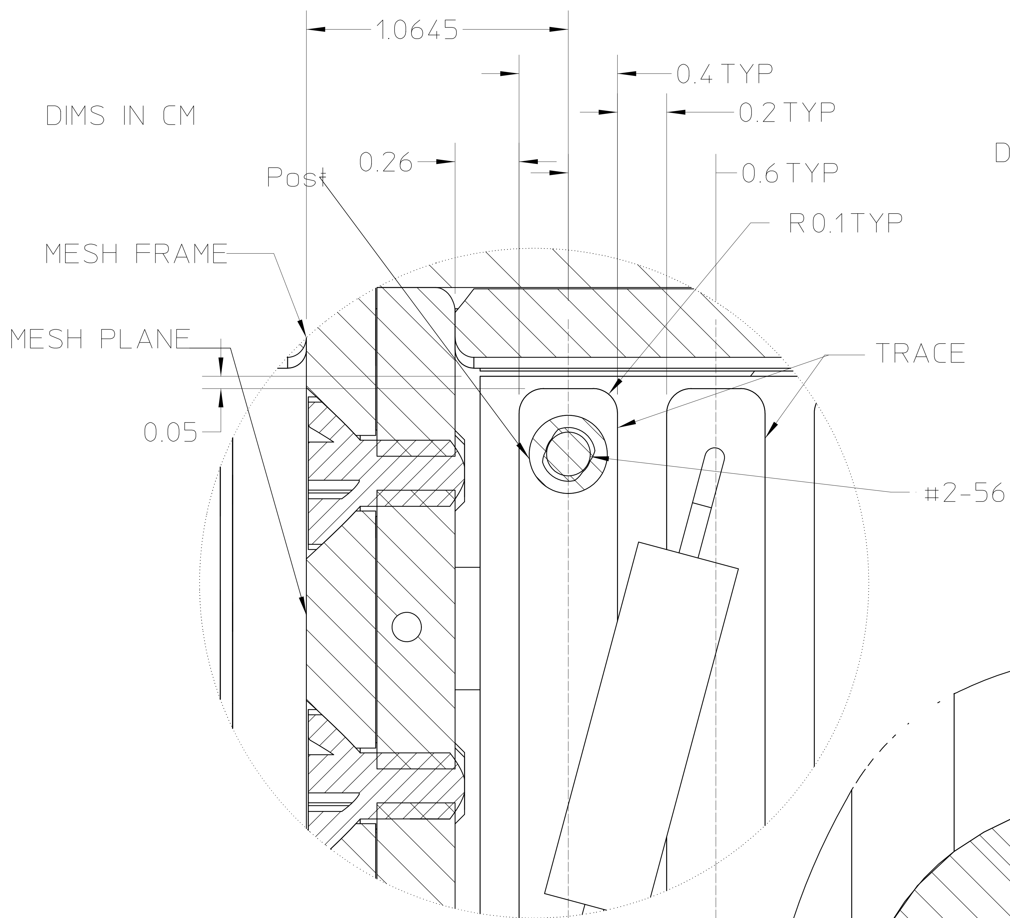
Detail3 SCALE 5:1
