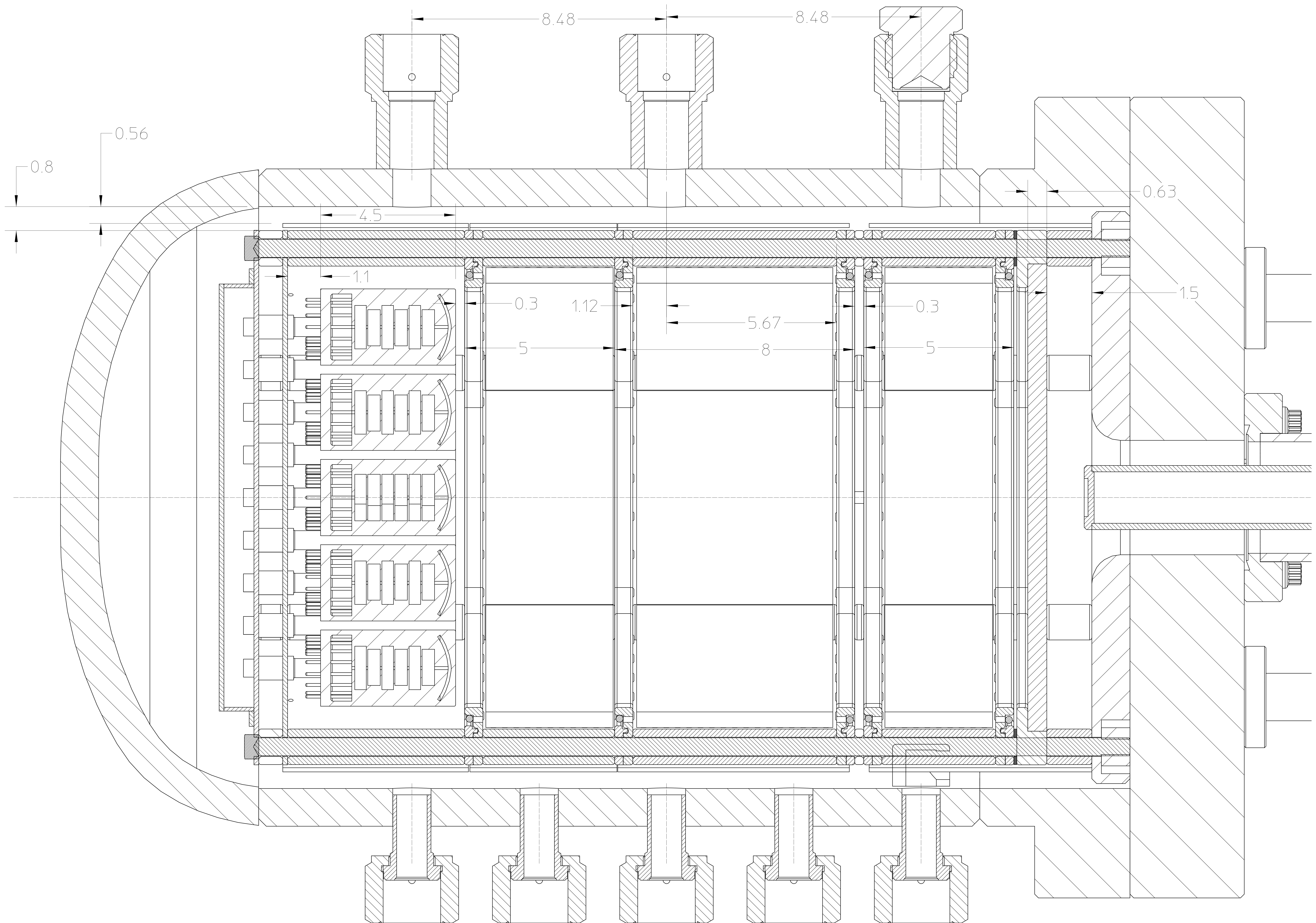
Section G-G
