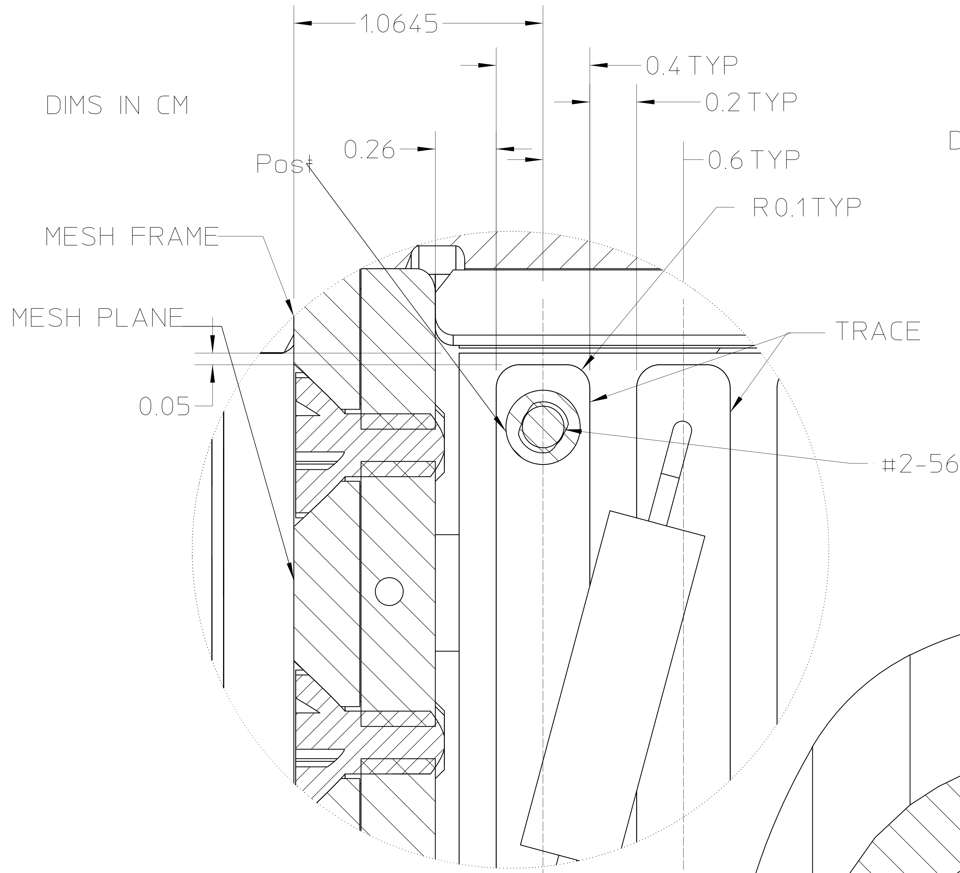
Detail3 SCALE 5:1
