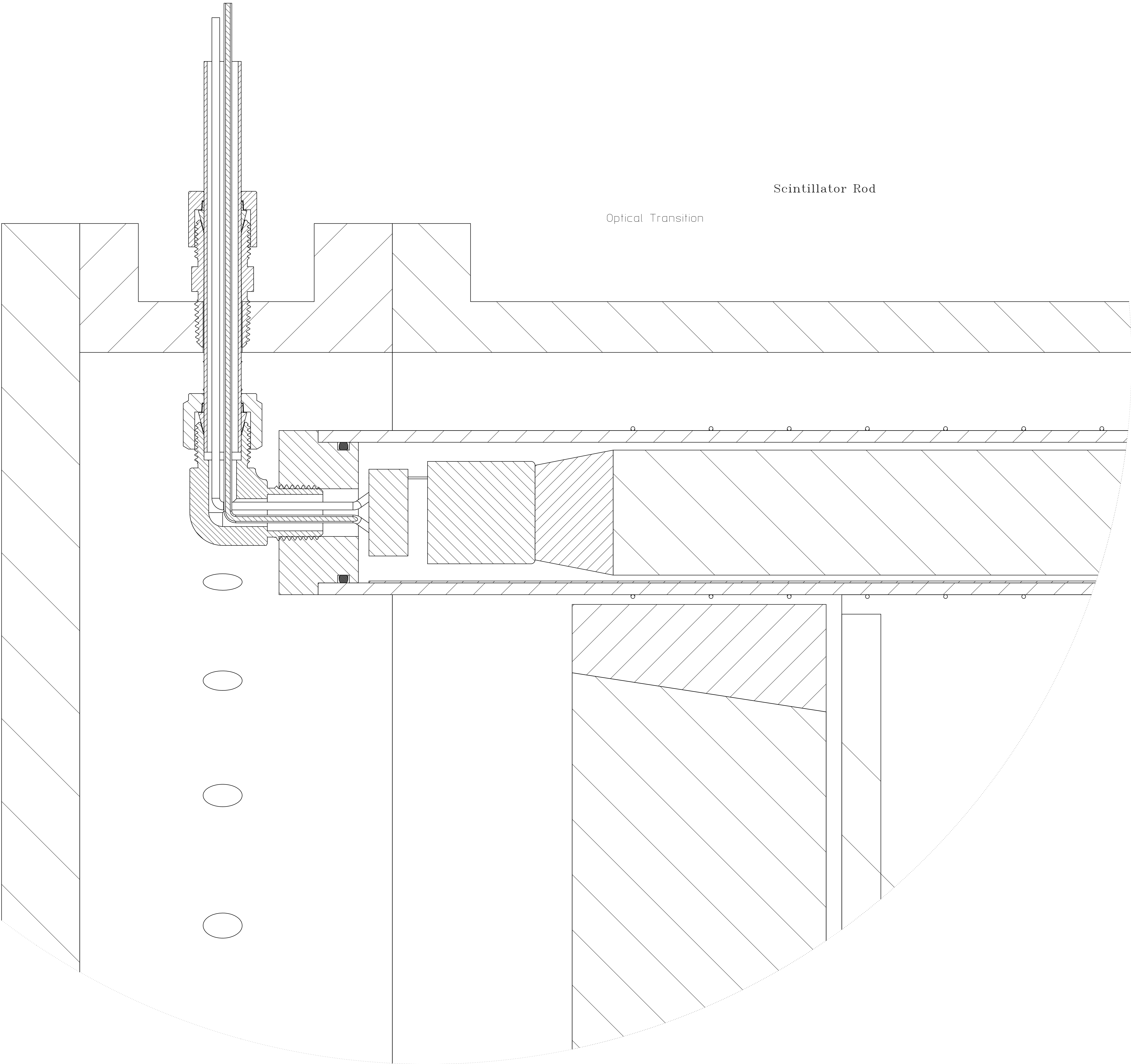
Detail1 SCALE 2:1
