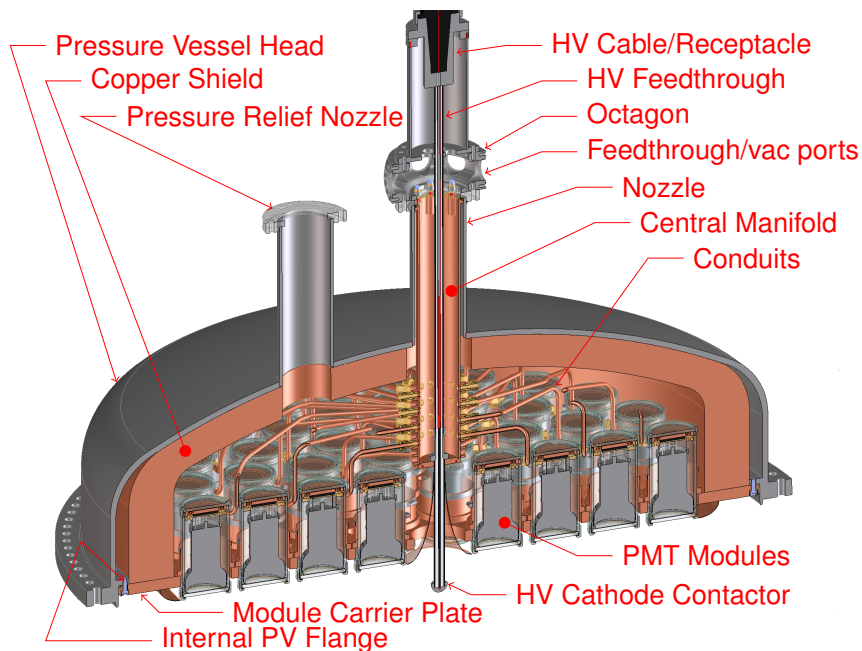
Figure 1: NEXT100, PMT Enclosure and Support System
