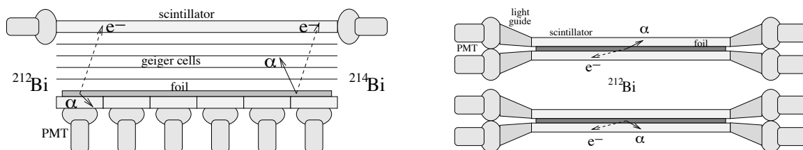
Figure 2: The 2 possible designs for the BiPo detector and the BiPo event signature: a prompt e^- and a delayed \alpha .
