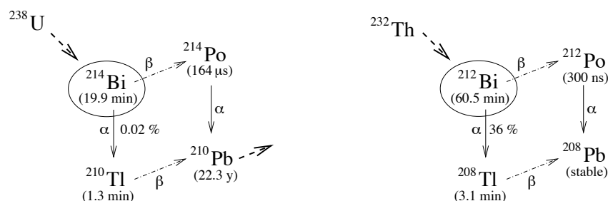
Figure 1: BiPo processes for ^{214}\text{Bi} and ^{208}\text{Tl} .
