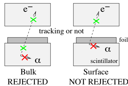
Figure 5: BiPo background from the scintillators : bulk and surface contamination. Crosses represent hits in scintillators.
