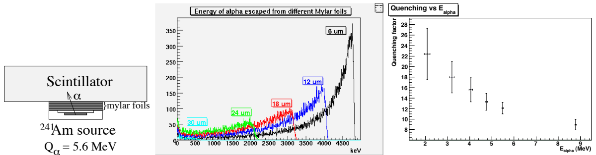
Figure 3: Measurement scheme - Energy spectrum of \alpha escaping the foil for different mylar's thickness ( 6 \mu\text{m} foils) - Measured quenching factors (the value at 8 MeV comes from a NEMO 3 measurement).
