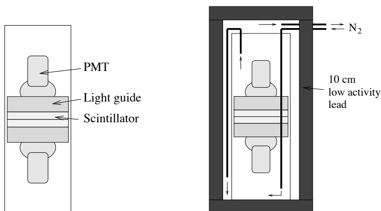
Figure 6: Scheme of a capsule of the BiPo-1 prototype and the first capsule with its own shielding in Canfranc.
