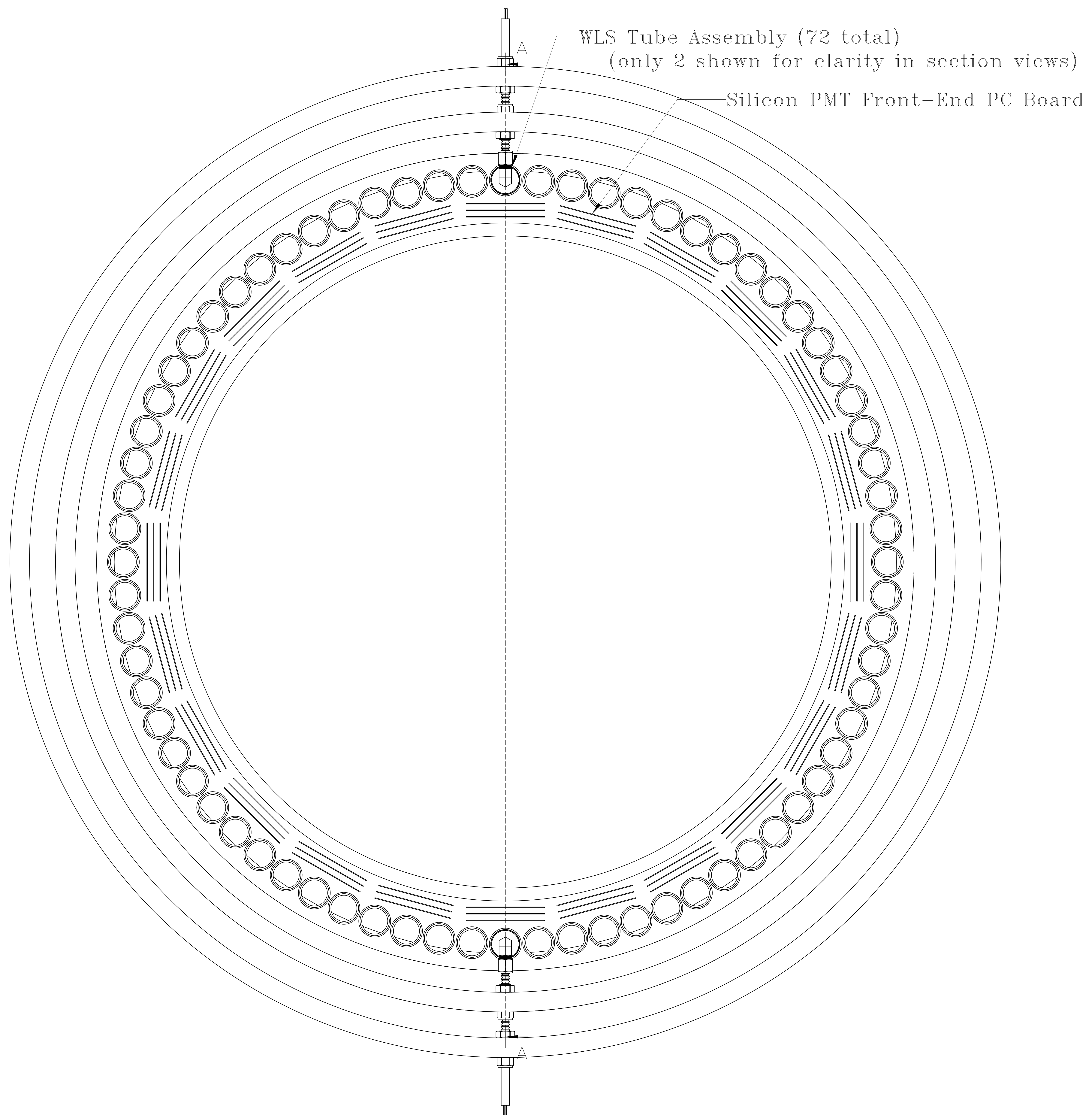
Top view, Pressure and Xenon vessel lids removed
