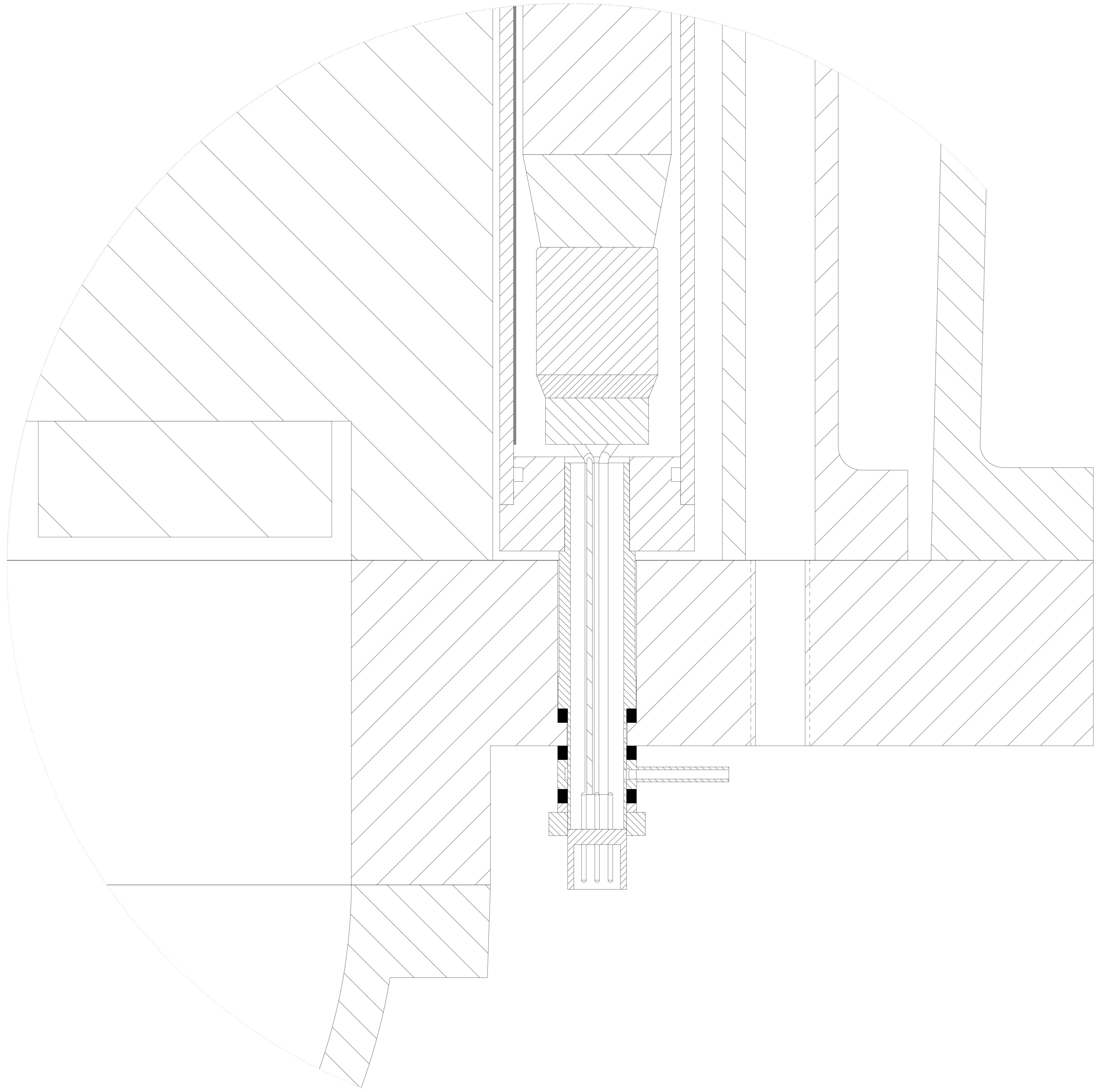
Detail1 SCALE 1:1
