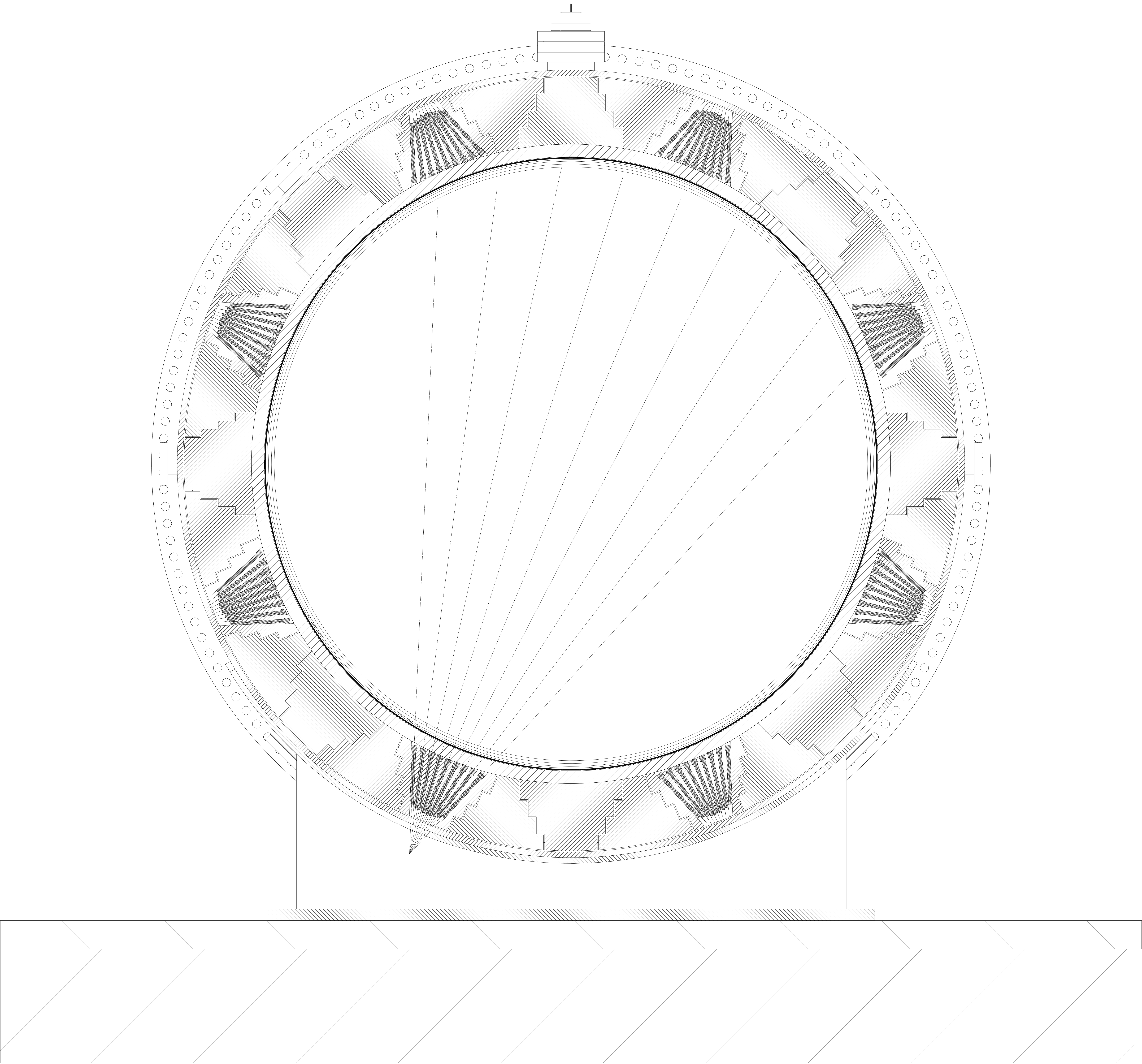
Section F-F
