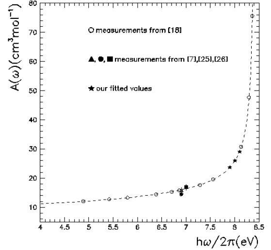
Figure 10. The dispersive behaviour of A(\omega) as a function of the photon energy \hbar\omega . Experimental measurements at higher densities are also shown (see text).
