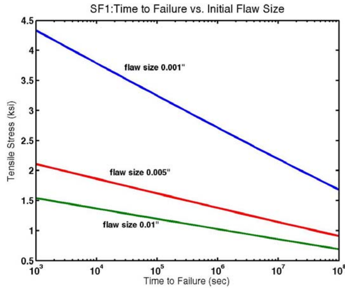
Figure 4.2 Time-to-Failure vs. Initial Flaw Size
