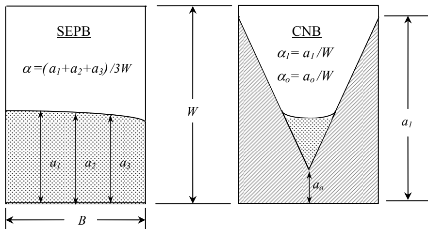
Figure 4.—Crack configurations and configuration for single-edge-precracked-beam and chevron-notch test specimens.
