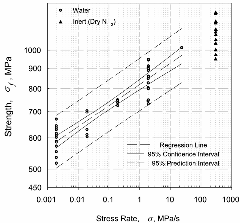
Figure 18.—Experimentally measured failure stress as a function of stress rate for the r -plane of sapphire in water. Four outlying specimens were censored.
