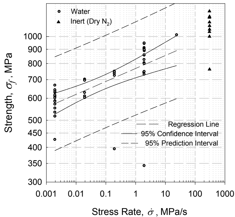
Figure 16.—Experimentally measured failure stress as a function of stress rate for the r -plane of sapphire in water.
