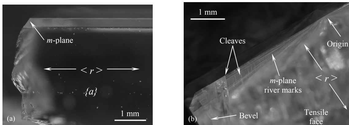
Figure 25.—(a) Side view of an r -plane test specimen (R3) showing typical m -plane crack extension from the mirror. Failure was from a long surface scratch. (b) Cleaves occurring away from the origin in an r -plane test specimen (R10) that failed at 733 MPa. River marks running along the m -plane are also apparent by looking through the tensile surface. Bifurcation did not occur along the tensile face.
