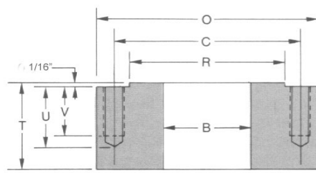
Flat Bottom
