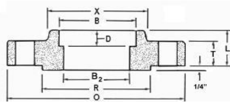
Socket Weld
