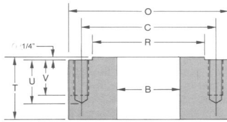
Flat Bottom
