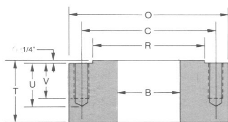
Flat Bottom
