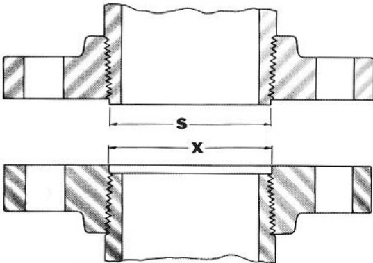
SMALL MALE AND FEMALE (on end of pipe)
