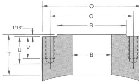
Shell/Head Mount
