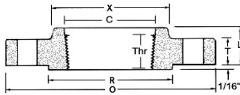
Threaded
