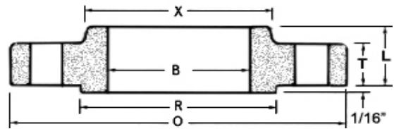
Slip-On
