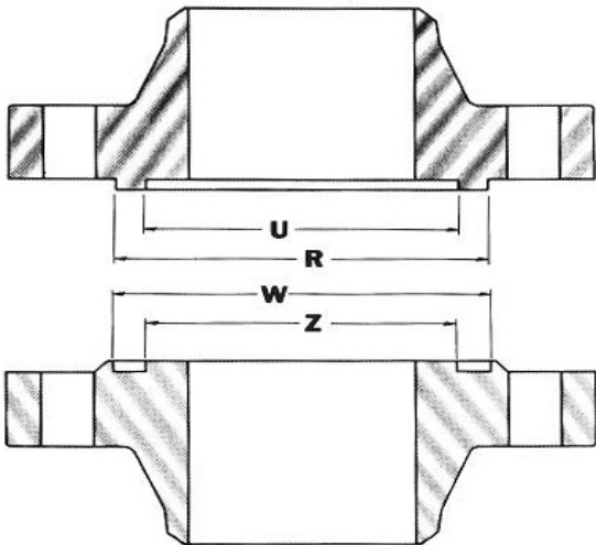
LARGE TONGUE AND GROOVE
