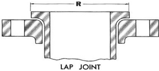
LAP JOINT
