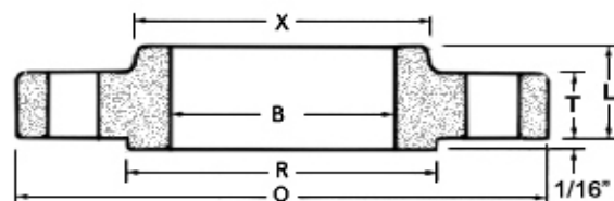
Slip-On
