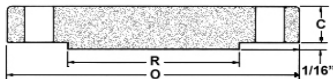
Blind
