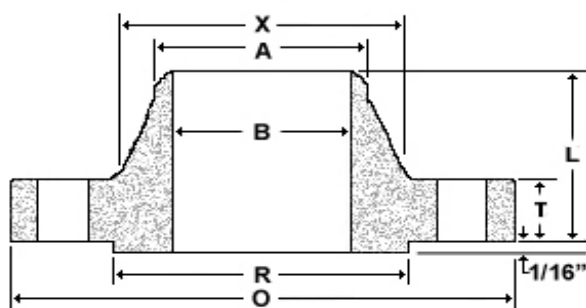
Weld Neck
