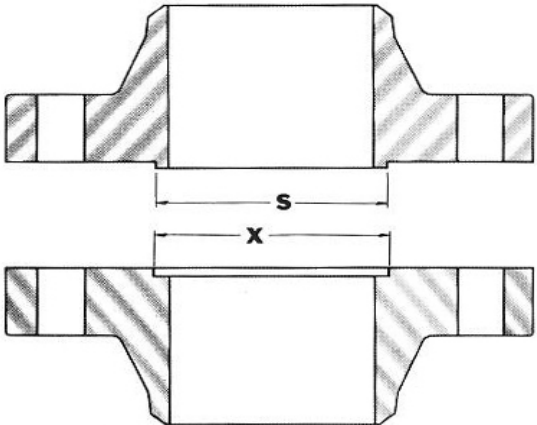
SMALL MALE AND FEMALE
