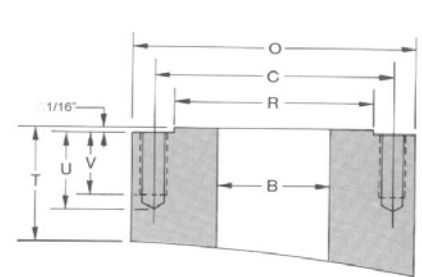
Tangential Mount
