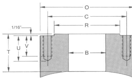
Shell/Head Mount
