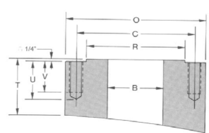
Tangential Mount
