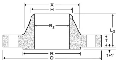
Weld Neck
