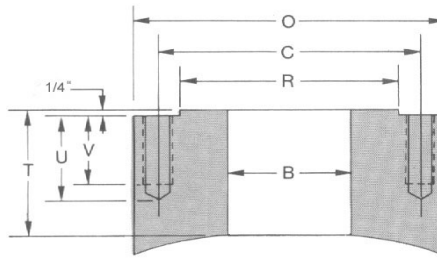
Shell/Head Mount
