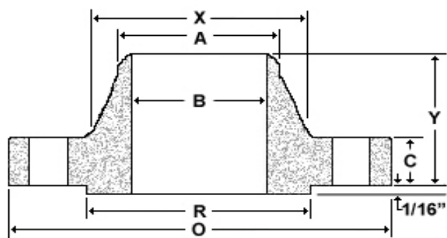
Weld Neck
