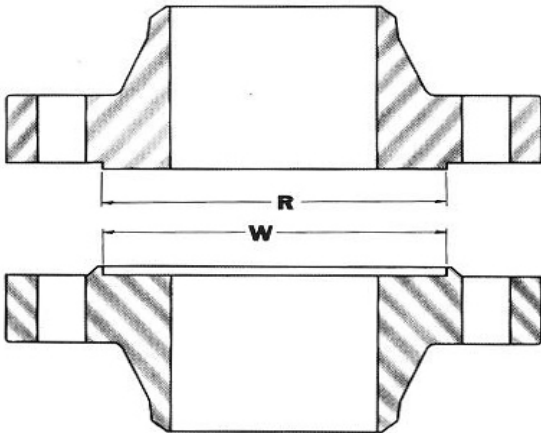
LARGE MALE AND FEMALE
