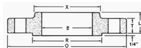
Slip-On
