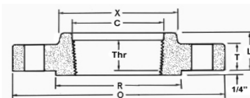
Threaded
