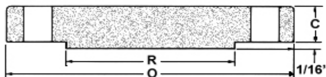
Blind
