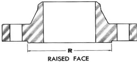
RAISED FACE
