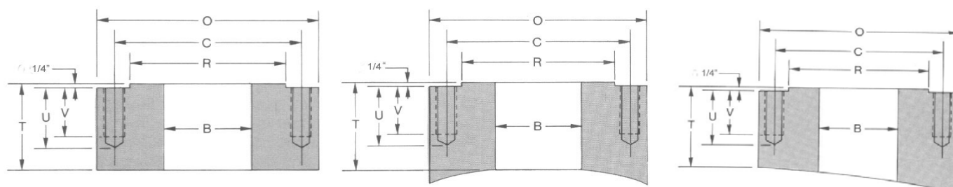
Flat Bottom
