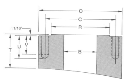
Tangential Mount
