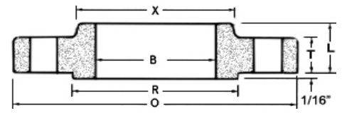
Slip-On
