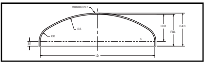
80/10 Dished
