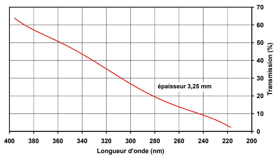
SPECTRE UV
