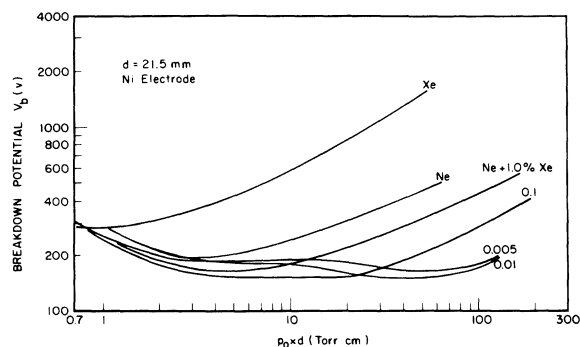
FIG. 6. Breakdown potential V_b vs p_0 d for Ne, Xe, and Ne-Xe mixtures.
