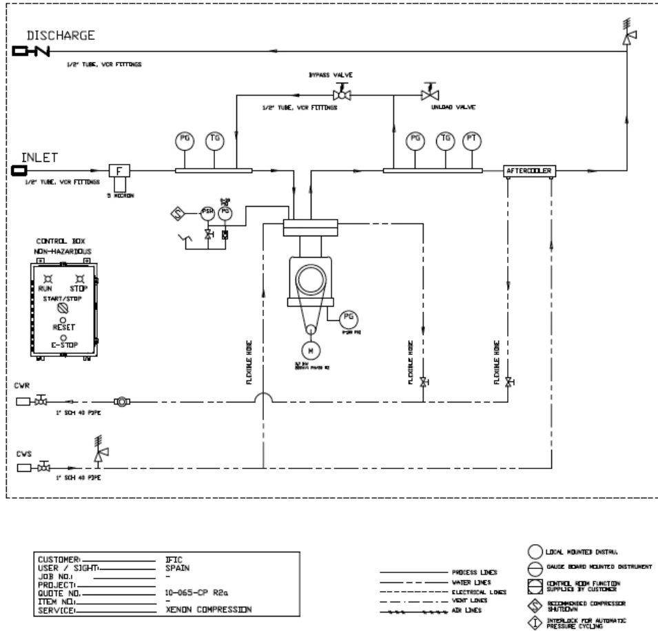
Figure 4: Schematic for the re-circulation pump.
