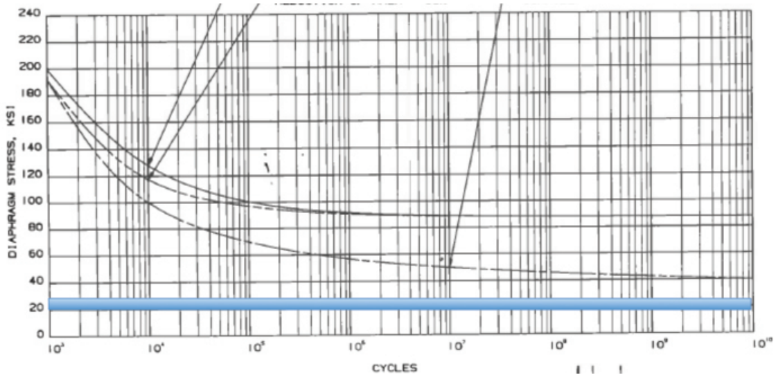
Figure 7: Failure curve for the single stainless steel diaphragm as a function of operating cycles. The pump is designed to operate in the shaded band. This translates into an expected time to failure of continuous operation in excess of 40 years.
