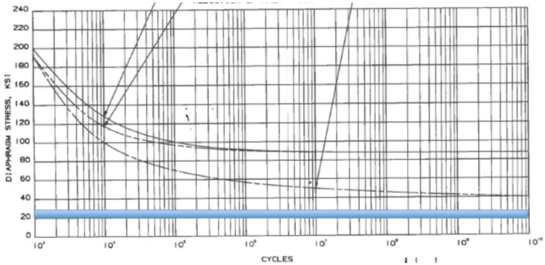
Figure 7: Failure curve for the single stainless steel diaphragm as a function of operating cycles. The pump is designed to operate in the shaded band. This translates into an expected time to failure of continuous operation in excess of 40 years.
