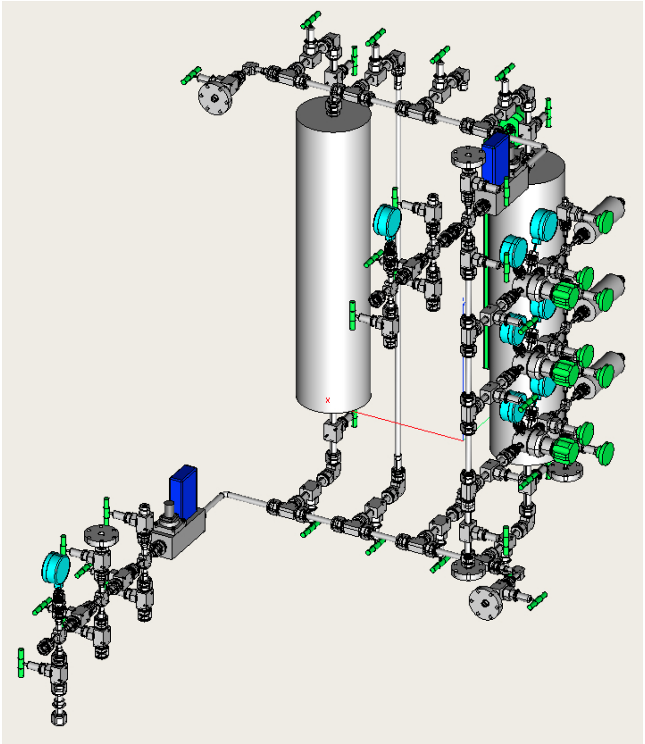
Figure 3: Three dimensional engineering model of the gas system piping.
