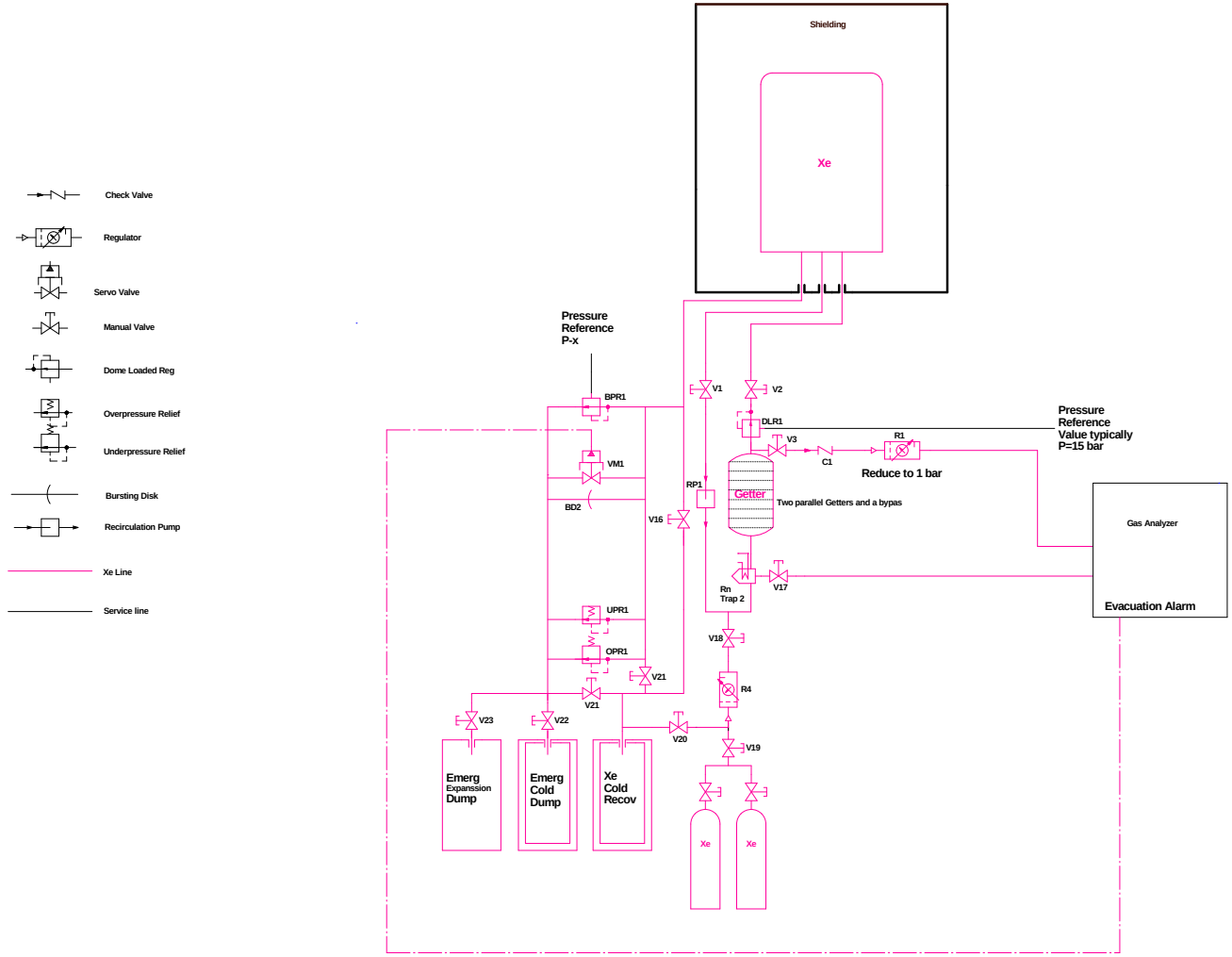
Figure 2: Schematic of the gas system.
