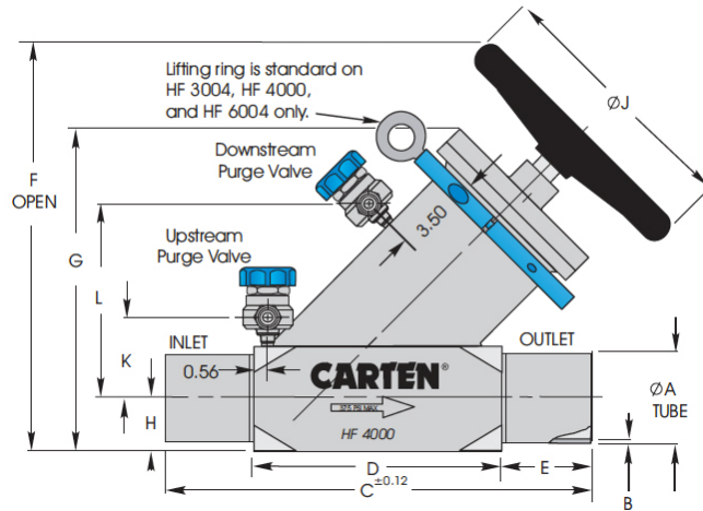
Figure 15: The HF4000 CARTEN valve.
