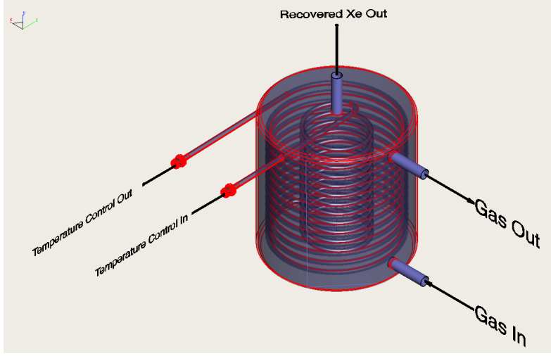
Figure 14: Example of a Xe cold trap.
