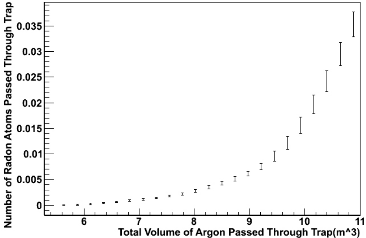
Figure 11: Total number of ^{222}\text{Rn} atoms that got through the trap as a function of the amount of argon gas for a 1 \text{ mBq/m}^3 assumed radon concentration in the argon supply.
