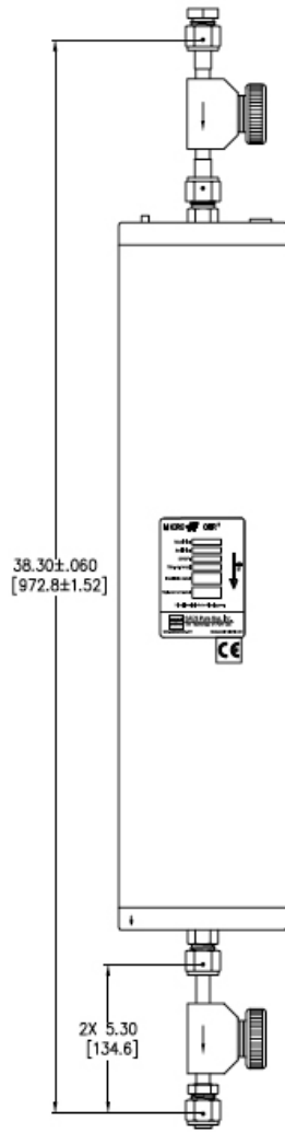
Figure 8: Drawing of the MC4500-902FV SAES Pure Gas getter, with VCR valves, to be used for the purification of the Xe. The gas system will contain two such parallel getters.
