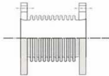
FLANGED END
