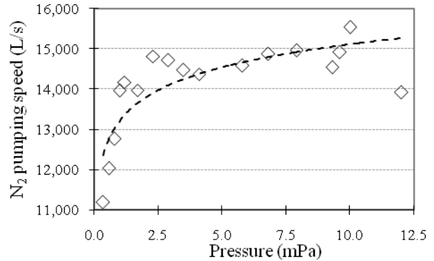
Figure 4: Test Cryopanel Pumping Speed vs. Pressure.
