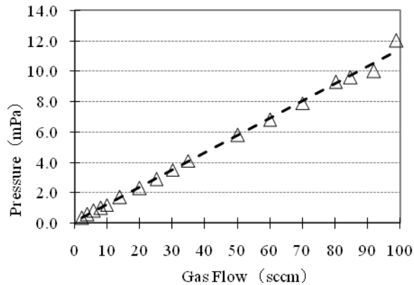
Figure 3: Test Cryopanel Pressure vs. Gas Flow.
