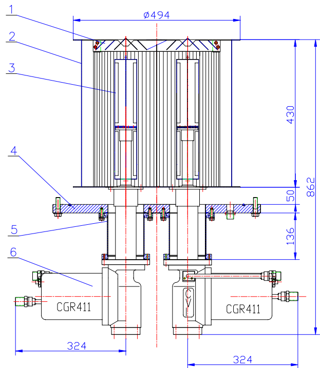
Figure 1: Plug-in Cryopump (1) half-chevron baffles, (2) shield, (3) cryopanel, (4) flange, (5) adapter, (6) GM refrigerator.
