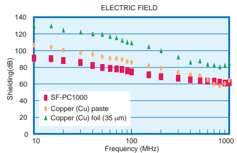
Fig. 6 Shielding characteristics (KEC method)
