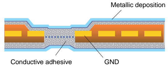
Fig. 3 Shielded FPC (Double-sided shielding)
