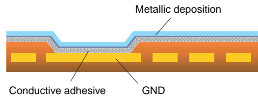
Fig. 2 Shielded FPC (Single-sided shielding)
