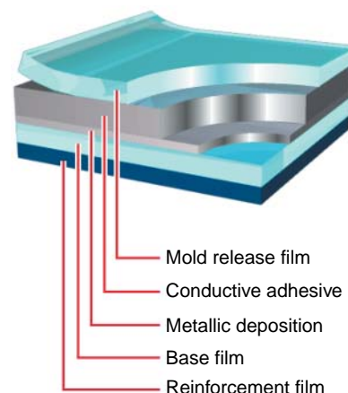
Fig. 1 Cross-sectional structure of the SF-PC1000
