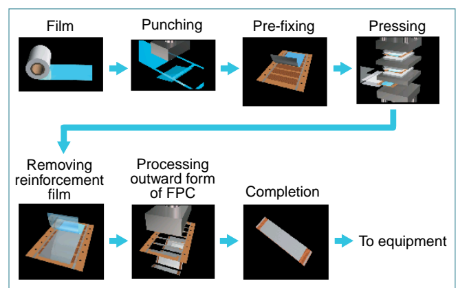
Fig. 9 Example of processing process for SF-PC1000
