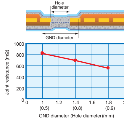
Fig. 8 Ground joint resistance (Double-sided shielding)
