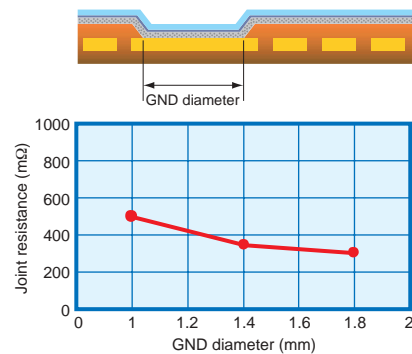
Fig. 7 Ground joint resistance (Single-sided shielding)
