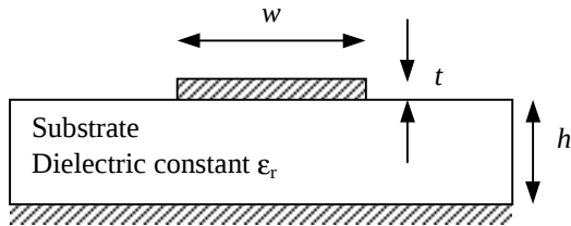
Figure 1 - Surface Microstrip
