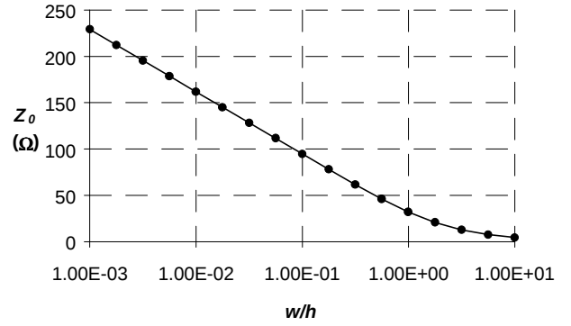
Figure 4 - Impedance for different relative width (Substrate \epsilon_r = 4.2 )
