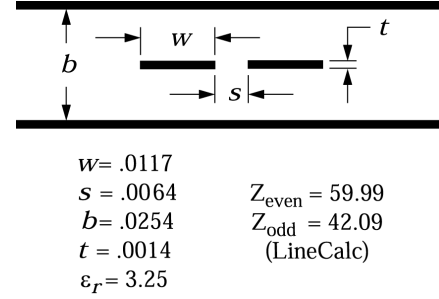
Fig. 7. Geometry and dimensions (inch) for simple coupled stripline test case.
