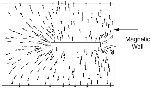
Fig. 9. E-field vectors for the even-mode, with all the lengths normalized to one value.
