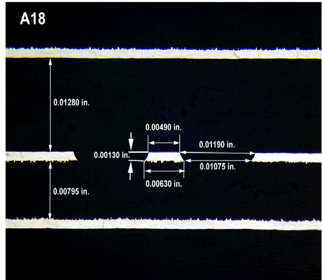
Fig. 14. Actual cross-section from an eight layer PC board, only three of the metal layers are shown.
