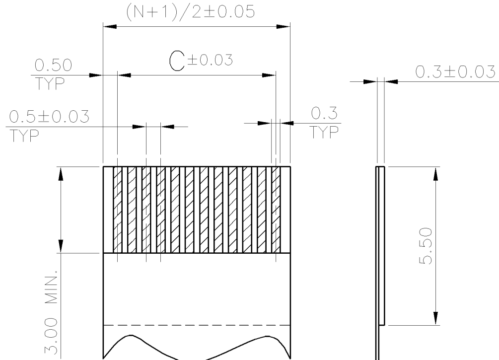
RECOMMENDED FPC/FFC LAYOUT (N = NO. OF CONTACTS)
