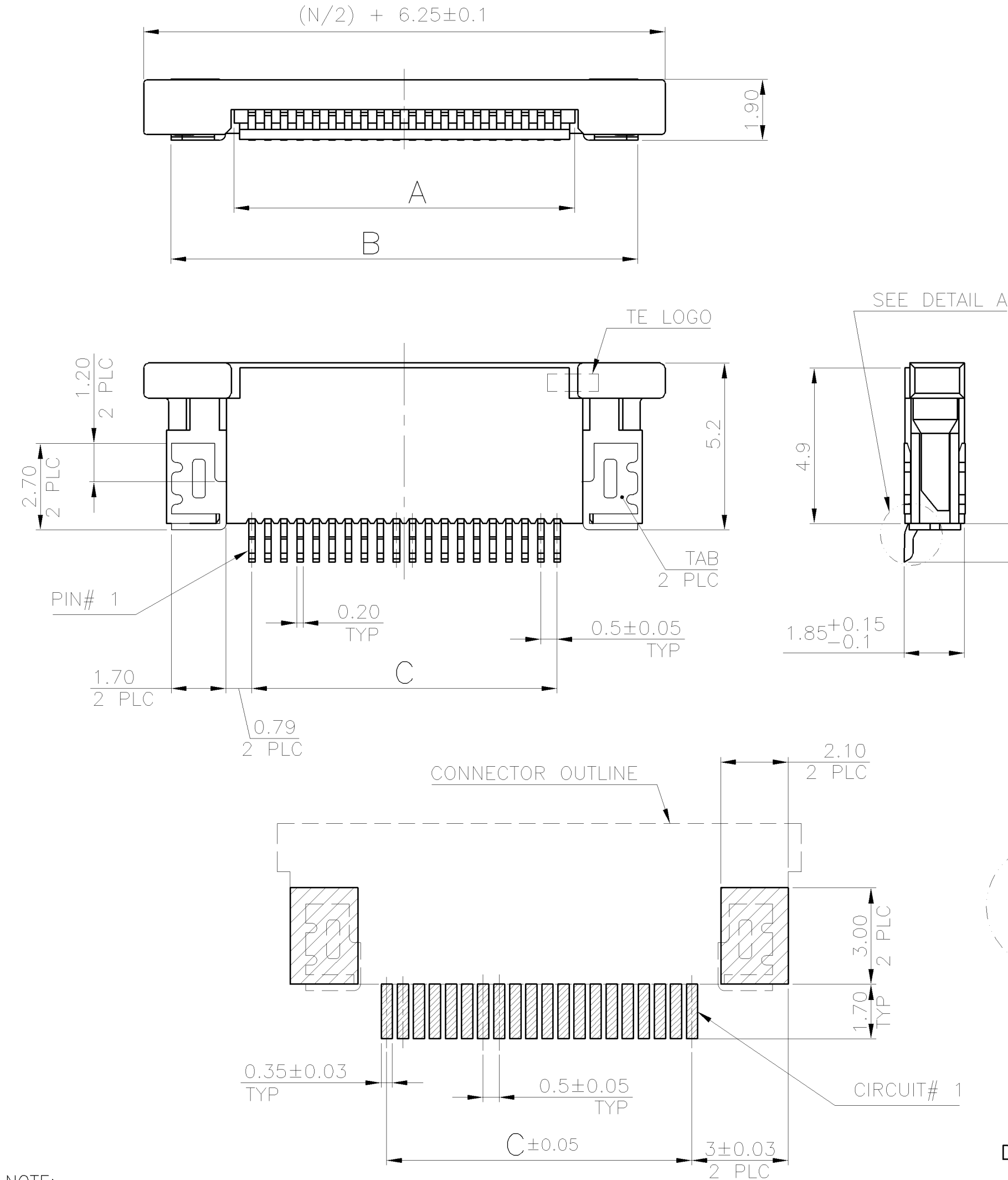
RECOMMENDED PCB LAYOUT
