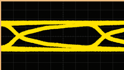
Eye Pattern
