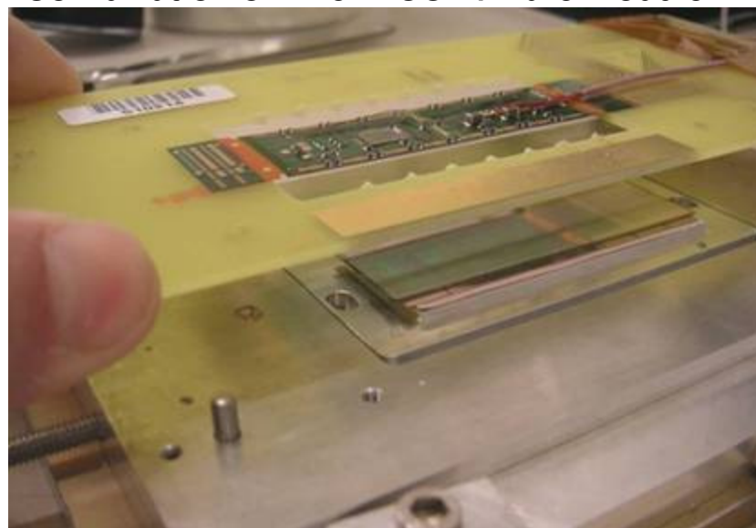
Combination of “FlexMCC” + Bare module
