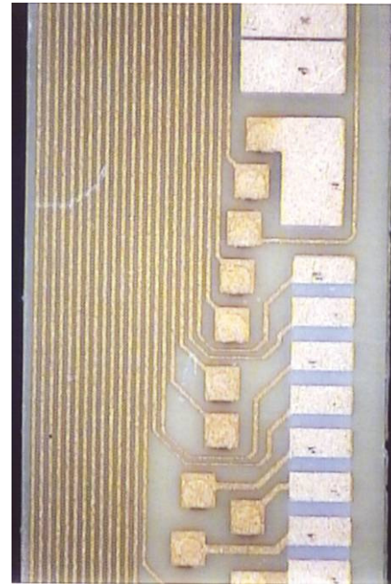
20 \mu m thin film traces
