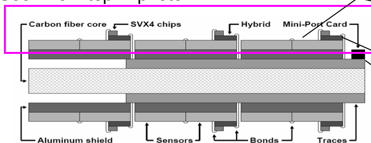
Simplified stave side view (not to scale)
