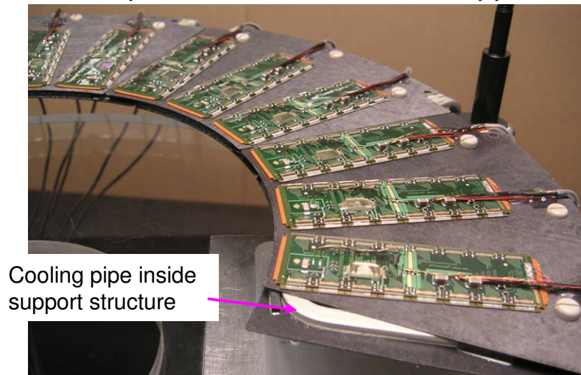
Atlas pixel modules on a disk support
