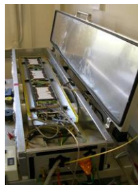
Single rod test
