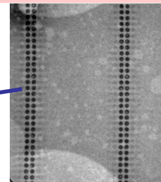
Xray of bumps
