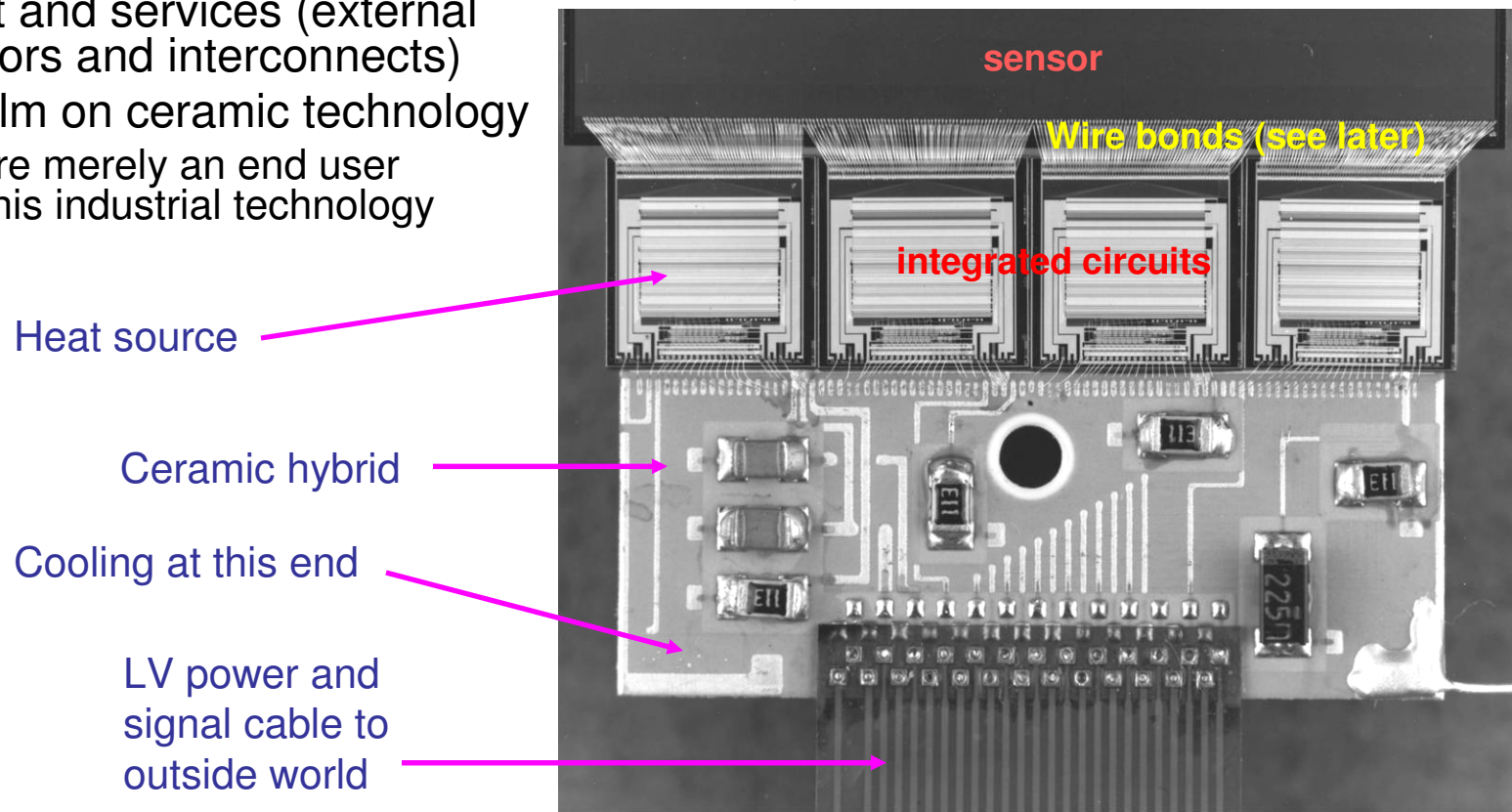
Hybrid at end of SVX ladder (1990)
