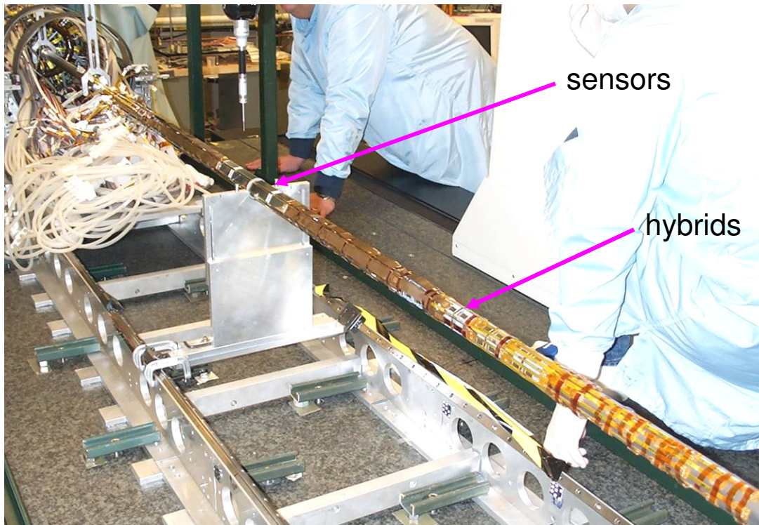
CDF Layer 00 (instrumented beam pipe)
