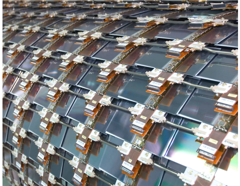
Atlas SCT modules on a support cylinder
