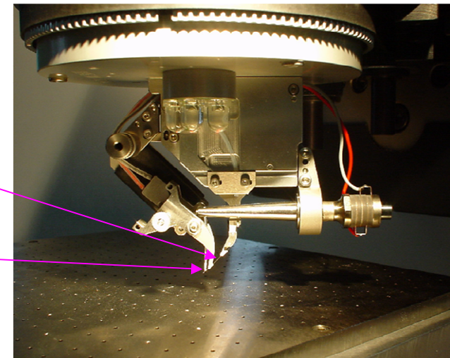
Bonding head
