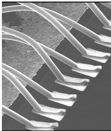
Bottom view of wire in wedge
