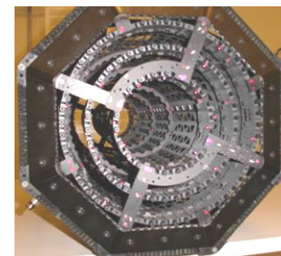
ATLAS pixel barrel
