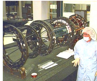
CDF-II ISL frame
