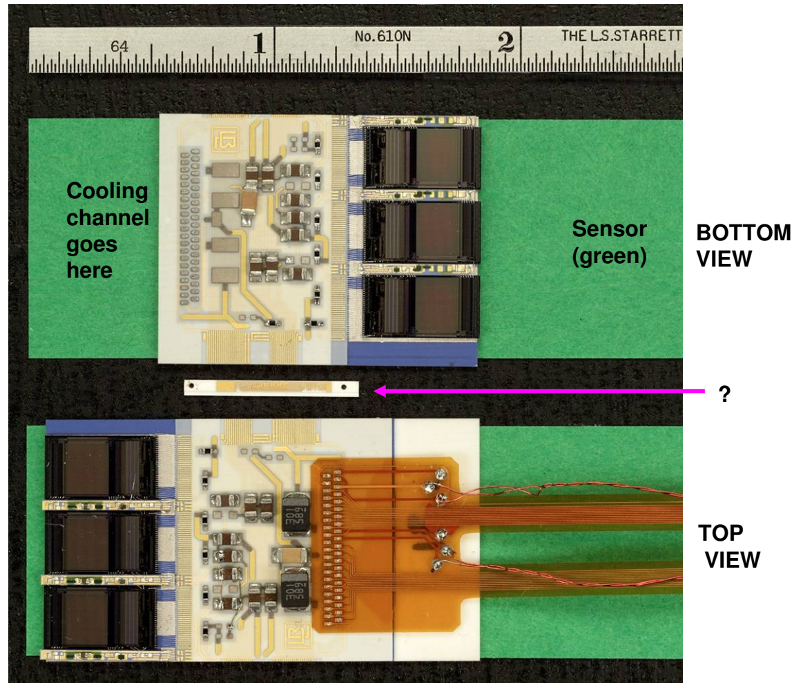
Prototype hybrids for SVX-II detector
