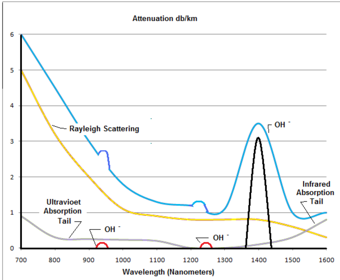
Figure 22. - Fiber losses.
