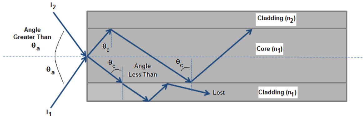
Figure 12. - How a light ray enters an optical fiber.
