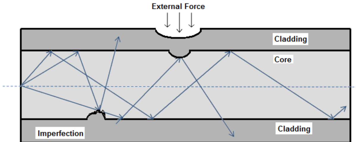
Figure 24. - Microbend loss.
