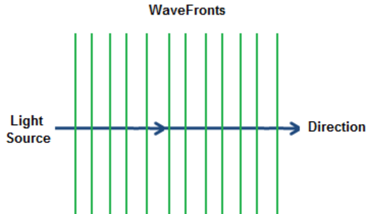
Figure 15. - Plane-wave propagation.
