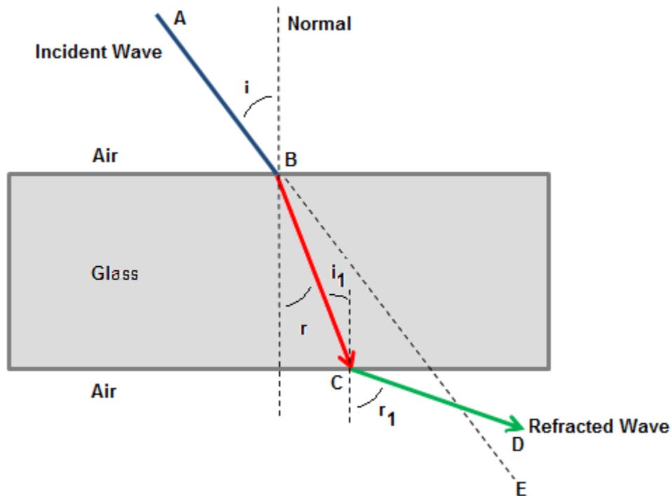
Figure 6. - Refraction of a wave.
