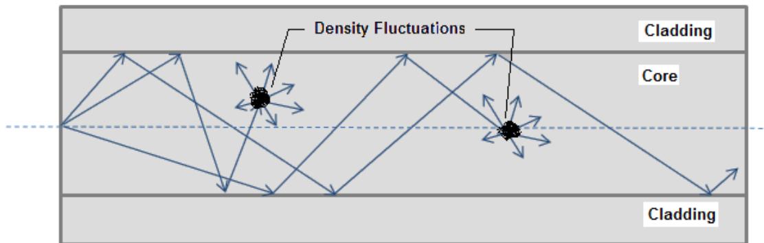
Figure 23. - Light scattering.
