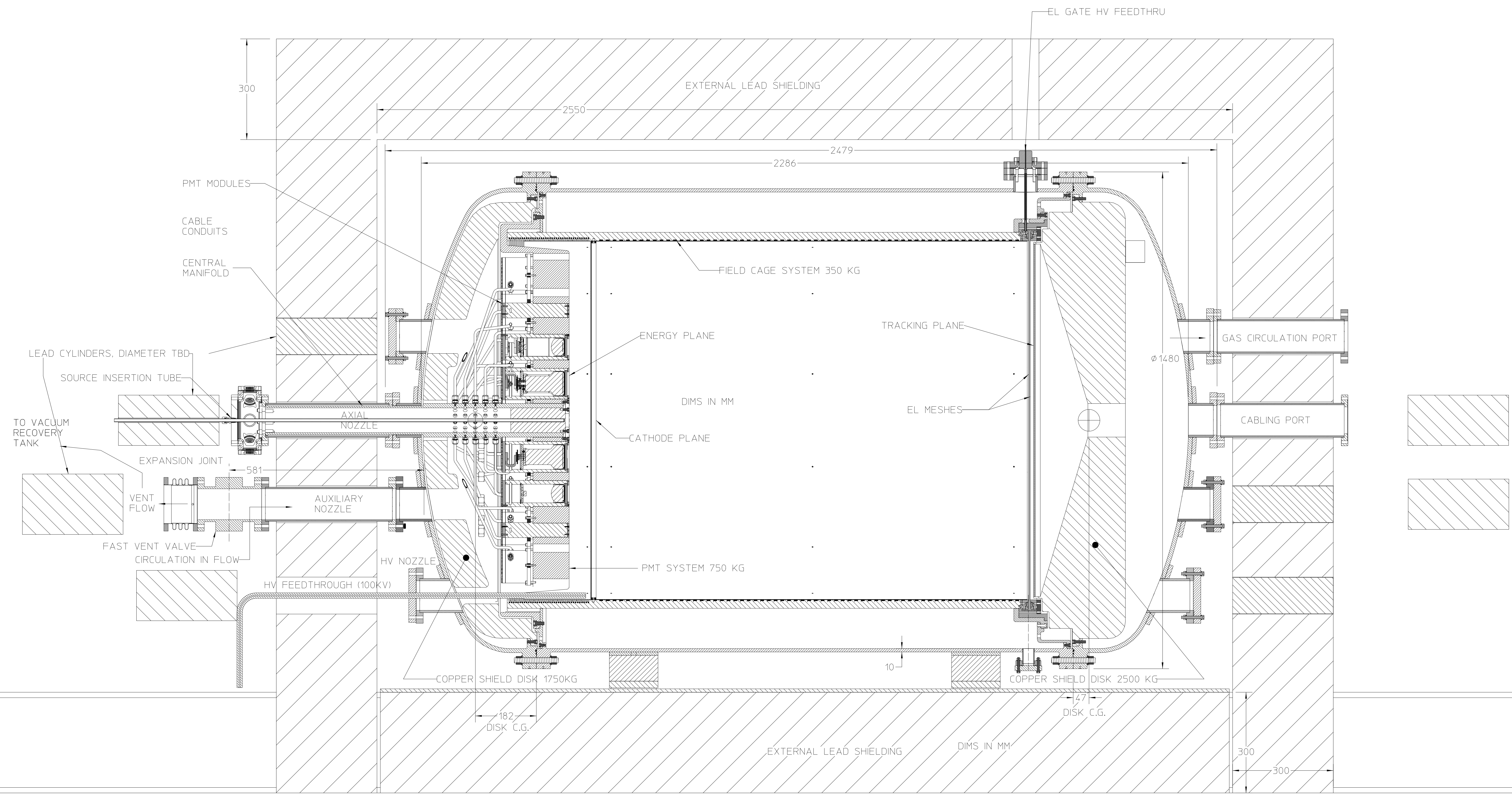
Section C-C
