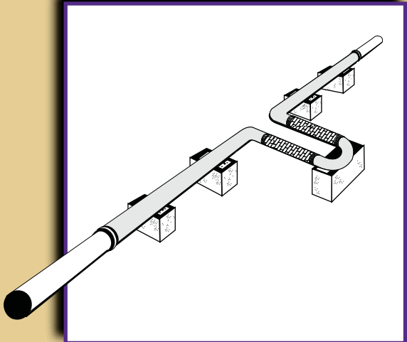
Plastic Pipe. Typically has much greater coefficients of expansion than steel and is more brittle. The ML Loop with its low spring rate is ideal.
