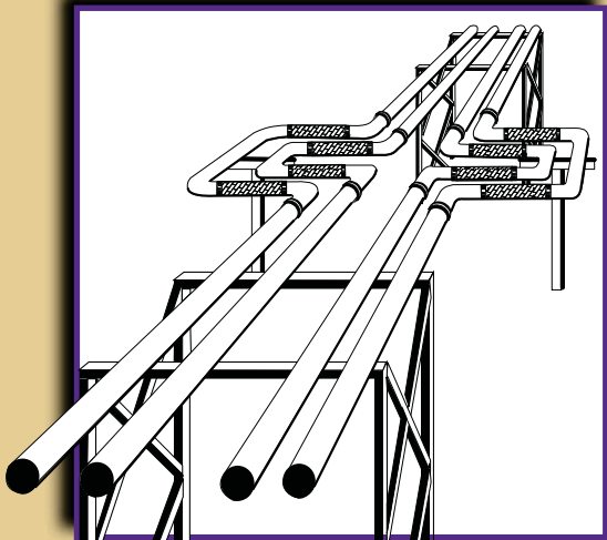
Elevated Pipe Runs. Reduced spring rates, anchor loads size, minimize the structural requirements of the pipe supports. Multiple hard pipe loops can be replaced by a single ML Loop.
