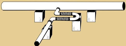
Branch line tie ins. In this installation the branch line can move perpendicular to the main line or the main line can move perpendicular to the branch without imposing any thrust loads.
