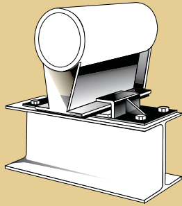
Pipe Supports. Because of the loops extreme flexibility guides are required within 4 pipe diameters before and after the loop. Teflon slide guides are recommended because they are impervious to atmospheric conditions. The teflon to stainless steel slide plates will never bind or gall. The slide guide also has the unique advantage of being able to support the piping so it can be used in place of pipe rollers for the entire pipe run.
