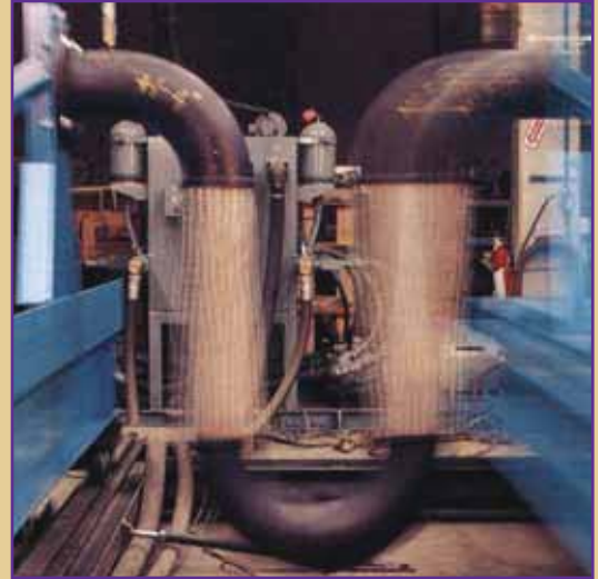
ML Loop Cycle Testing, WJE No. 941166, December 1994
