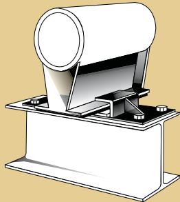
Pipe Supports. Because of the loops extreme flexibility guides are required within 4 pipe diameters before and after the loop. Teflon slide guides are recommended because they are impervious to atmospheric conditions. The teflon to stainless steel slide plates will never bind or gall. The slide guide also has the unique advantage of being able to support the piping so it can be used in place of pipe rollers for the entire pipe run.
