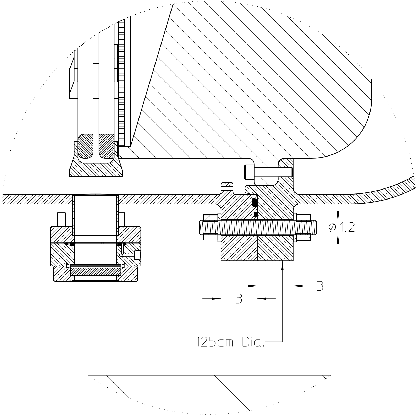
Double O-ring only (possible helicoflex capable) Design
