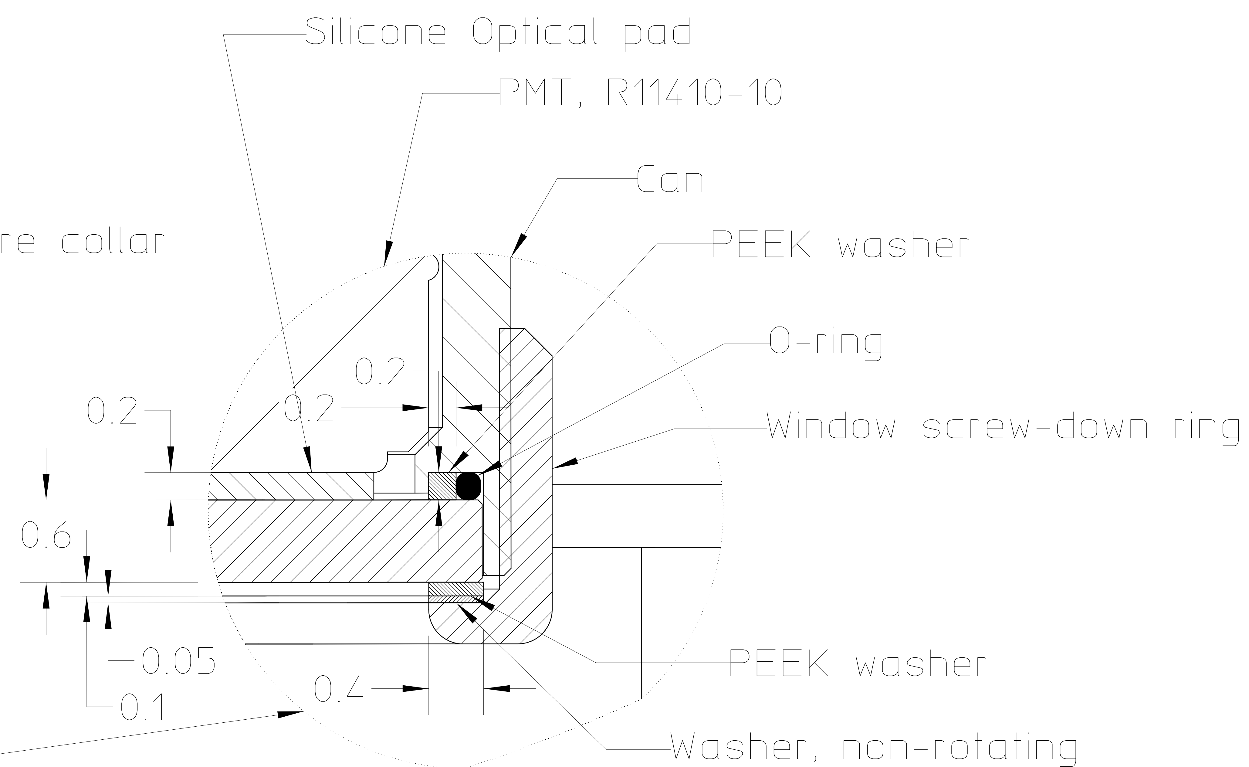
Detail3 SCALE 2:1
