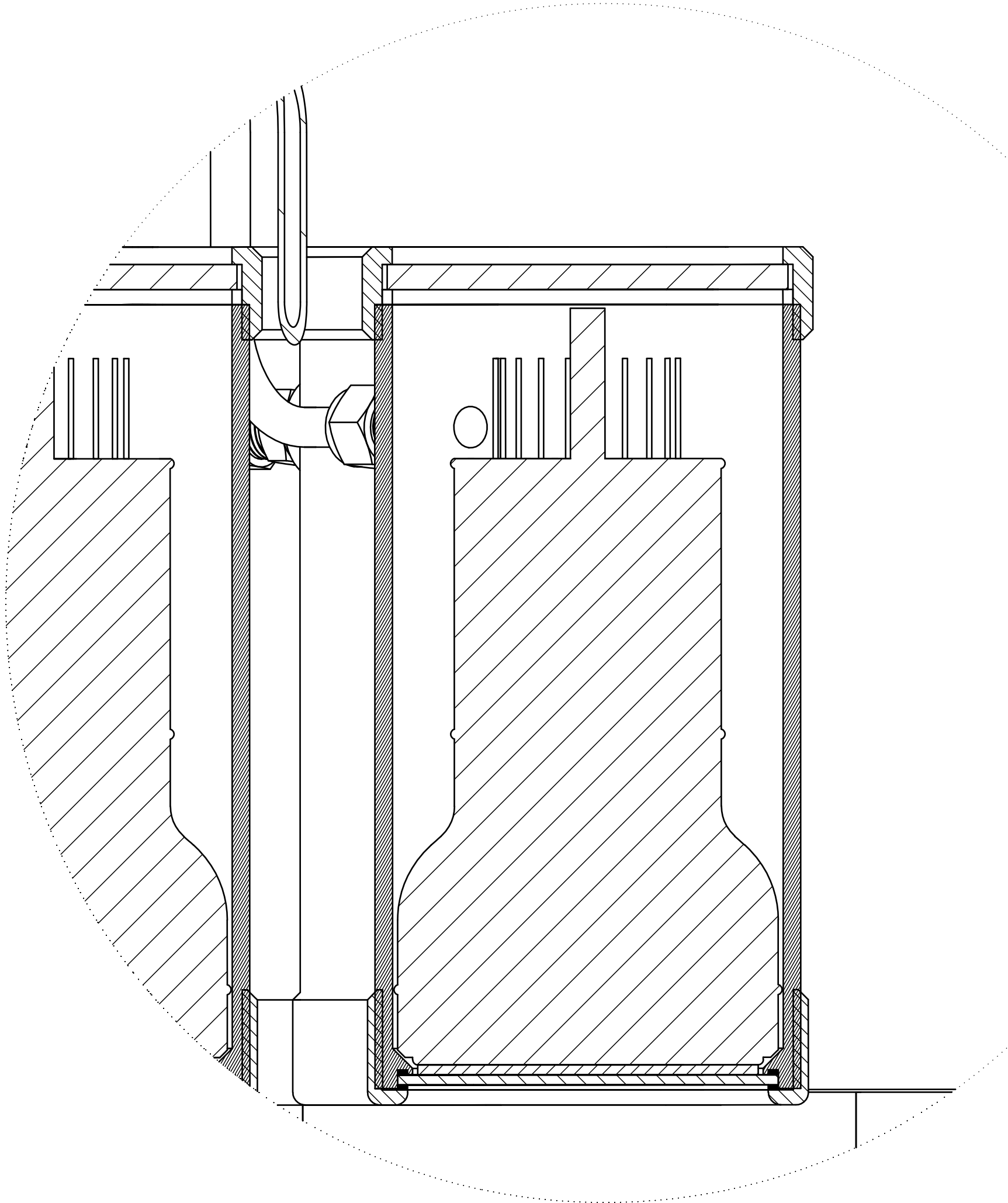
Detail2 SCALE 1:2
