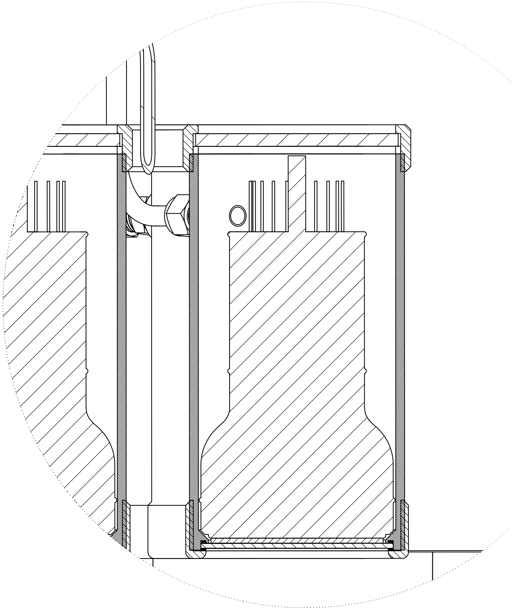
Detail2 SCALE 1:2
