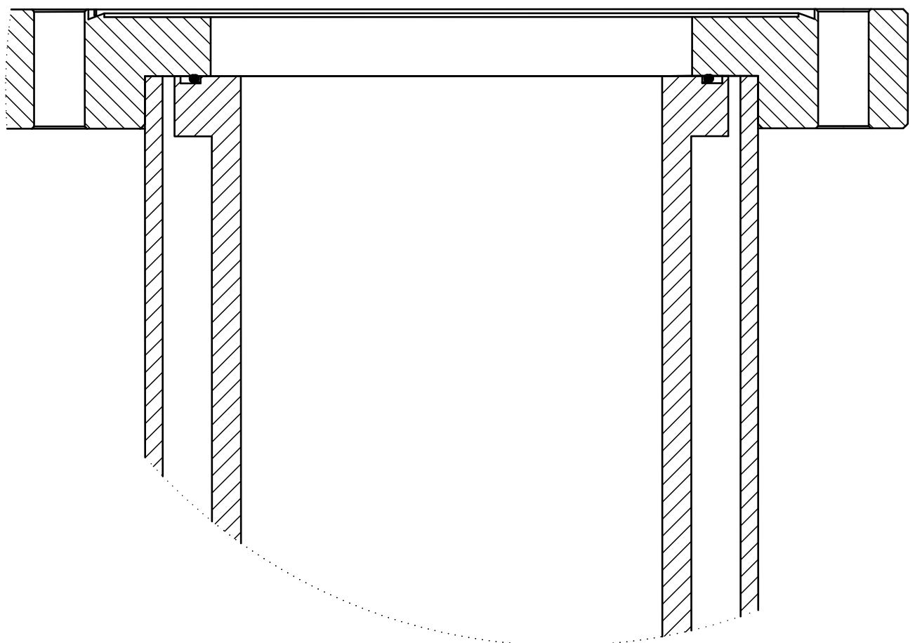
Detail1 SCALE 1:2
