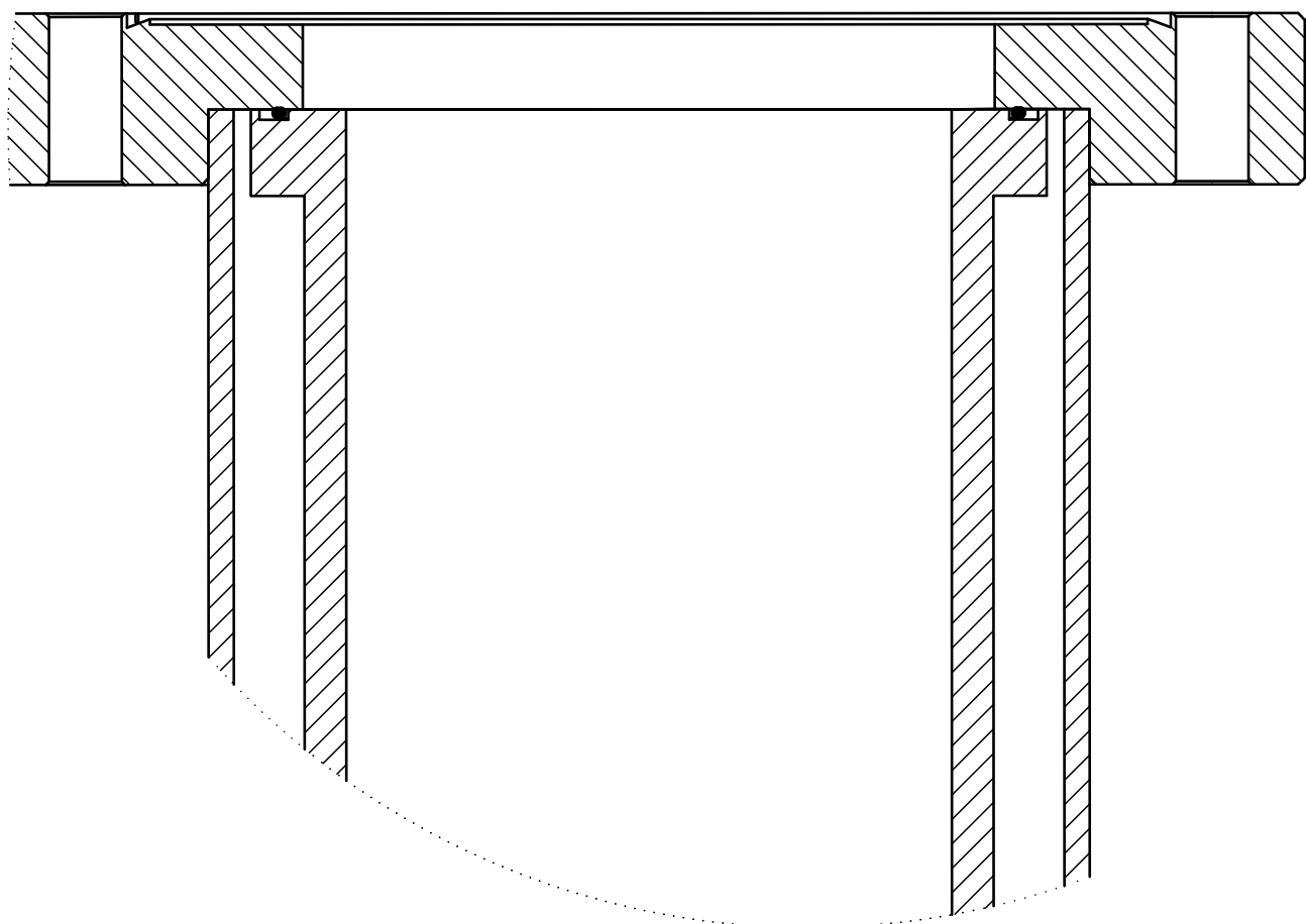
Detail1 SCALE 1:2
