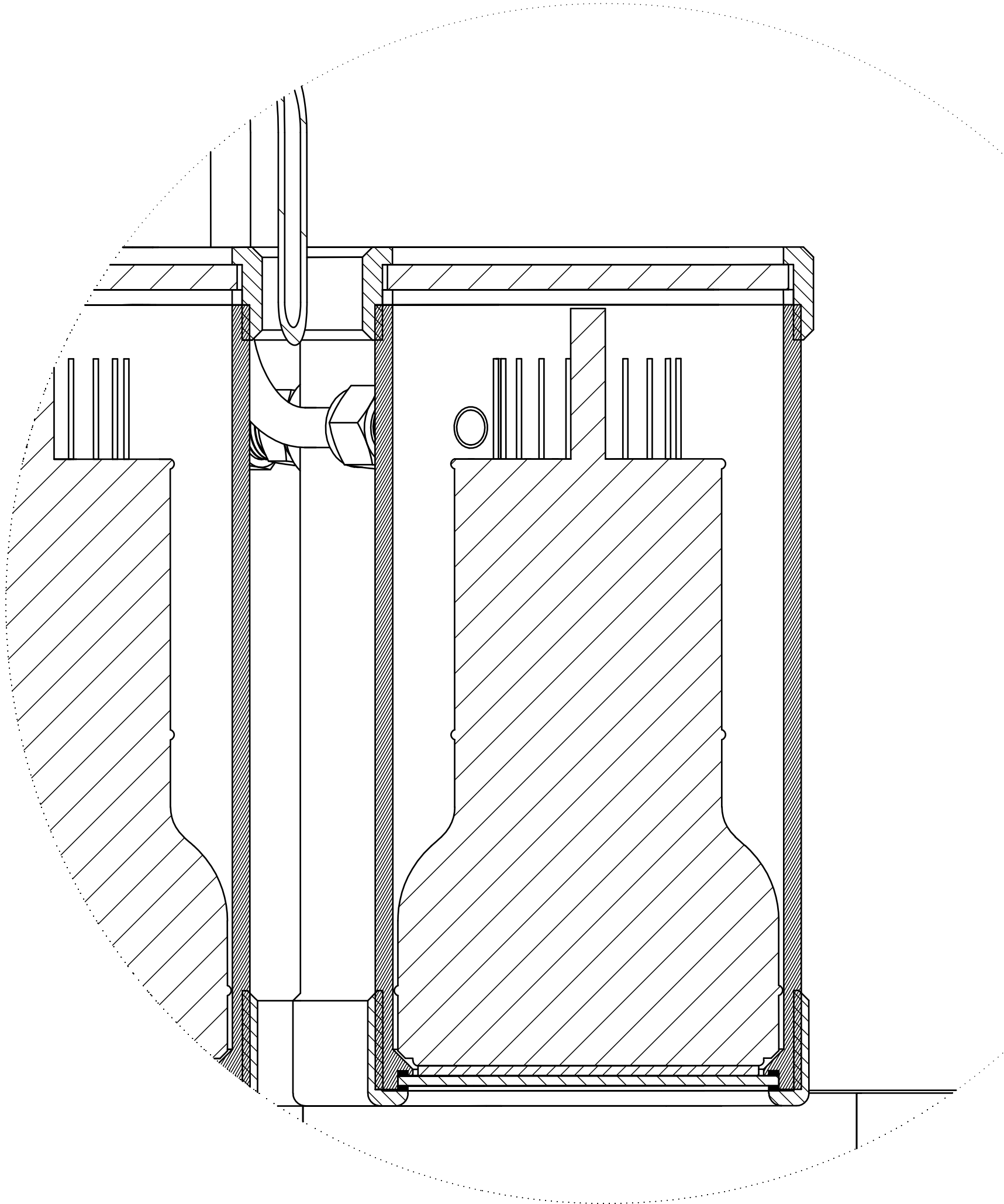
Detail2 SCALE 1:2
