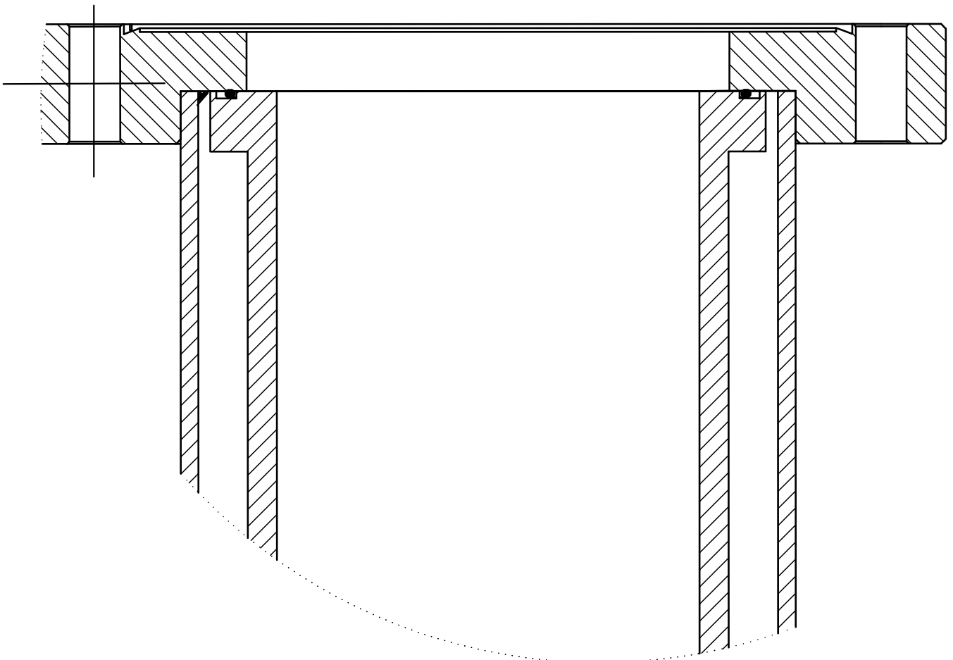
Detail1 SCALE 1:2
