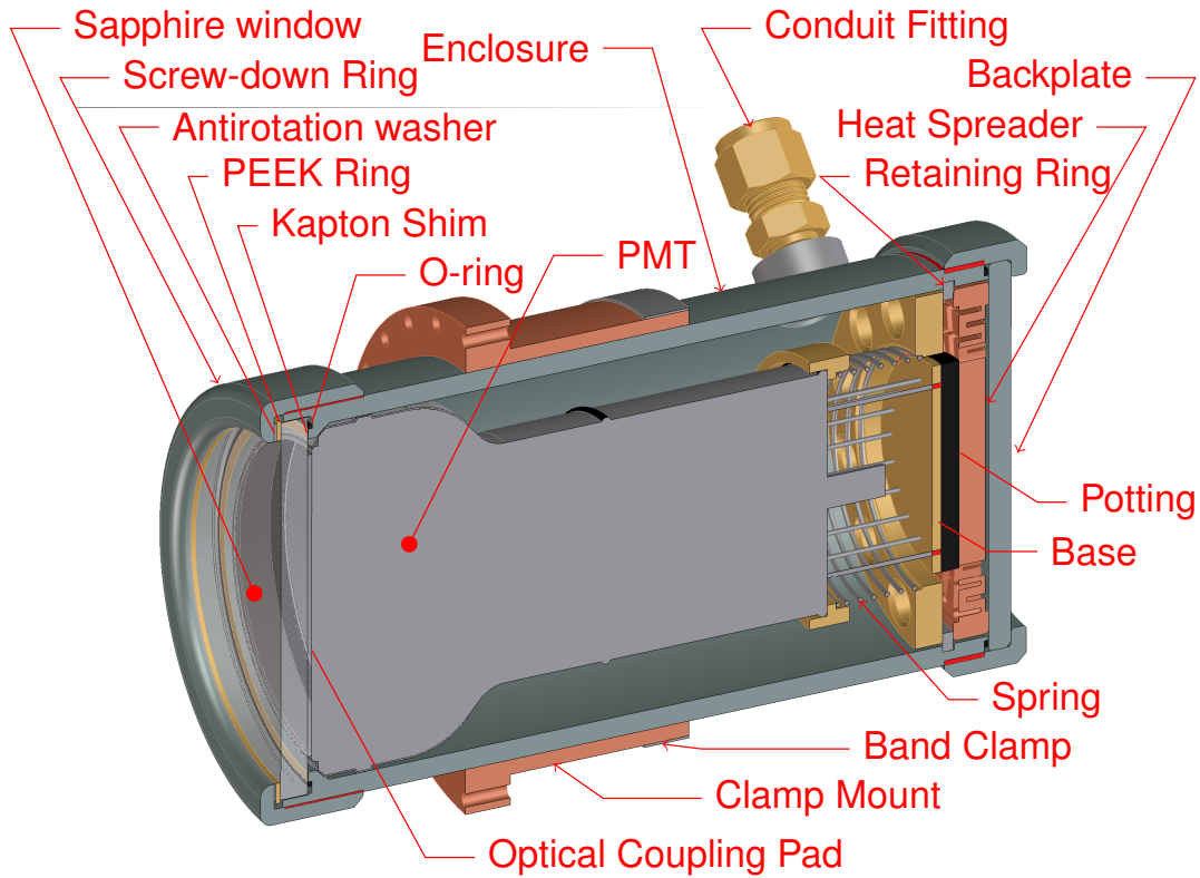
Figure 2: PMT Module
