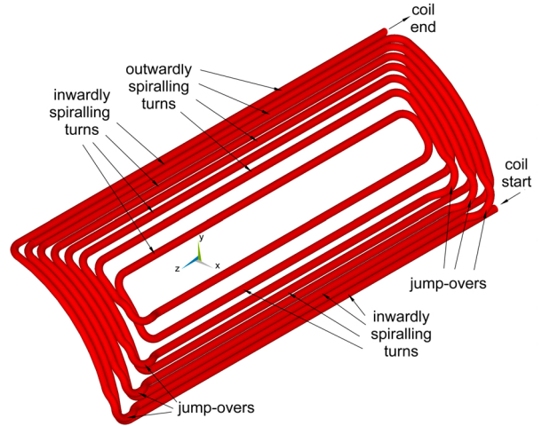
Fig. 2 Single Layer/Double Pancake Coil Design
