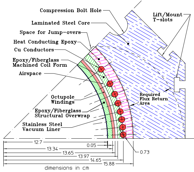
Fig. 1 Octant Cross-Section
