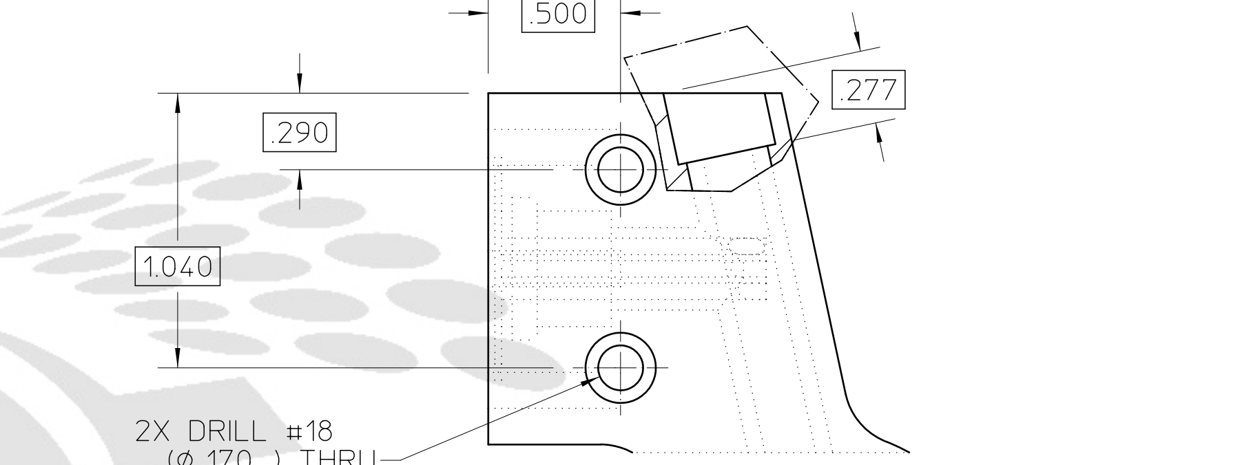
Detail 1 SCALE 2/1 STANDARD 1-1/2 MINI-CFF KNIFE EDGE
