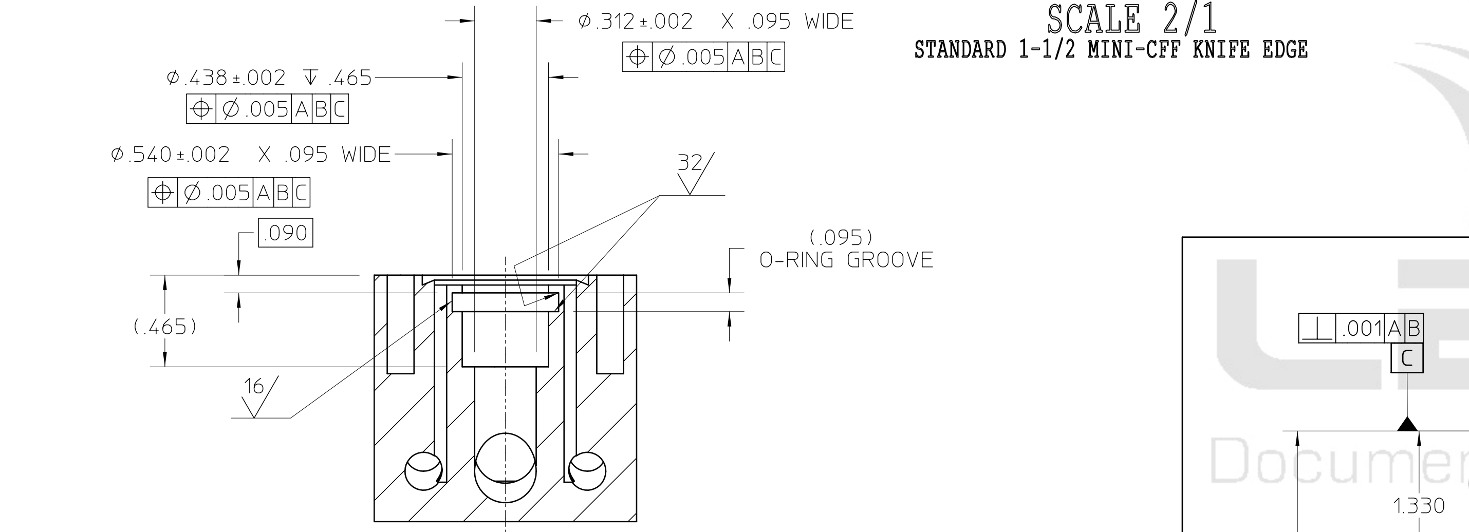
SECTION B-B SCALE 2/1 STANDARD 1-1/2 MINI-CFF KNIFE EDGE
