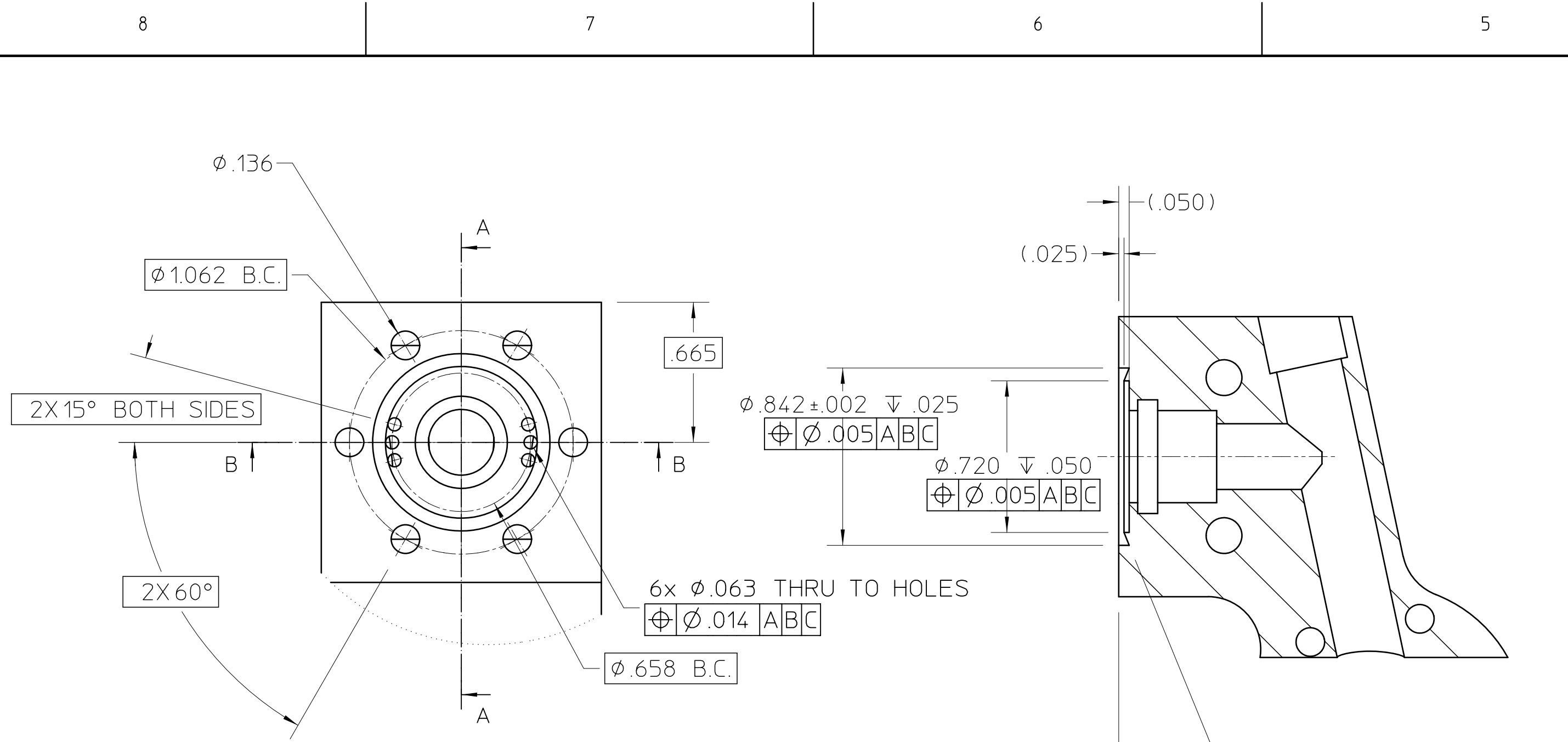
Detail 1 SCALE 2/1 STANDARD 1-1/2 MINI-CFF KNIFE EDGE
