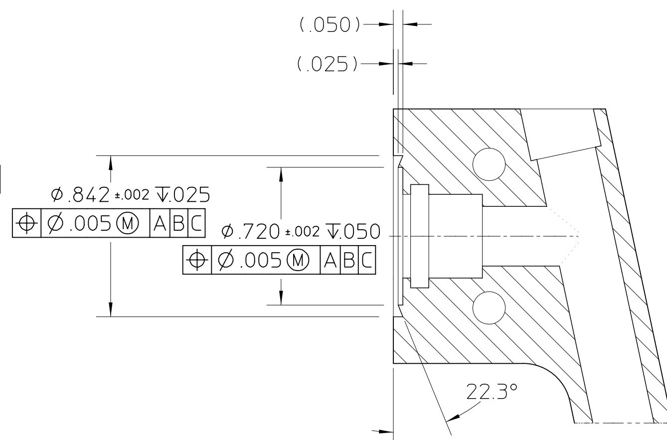
SECTION C-C TYP 3 PLACES SCALE 2/1 STANDARD 1-1/3 MINI-CFF KNIFE EDGE
