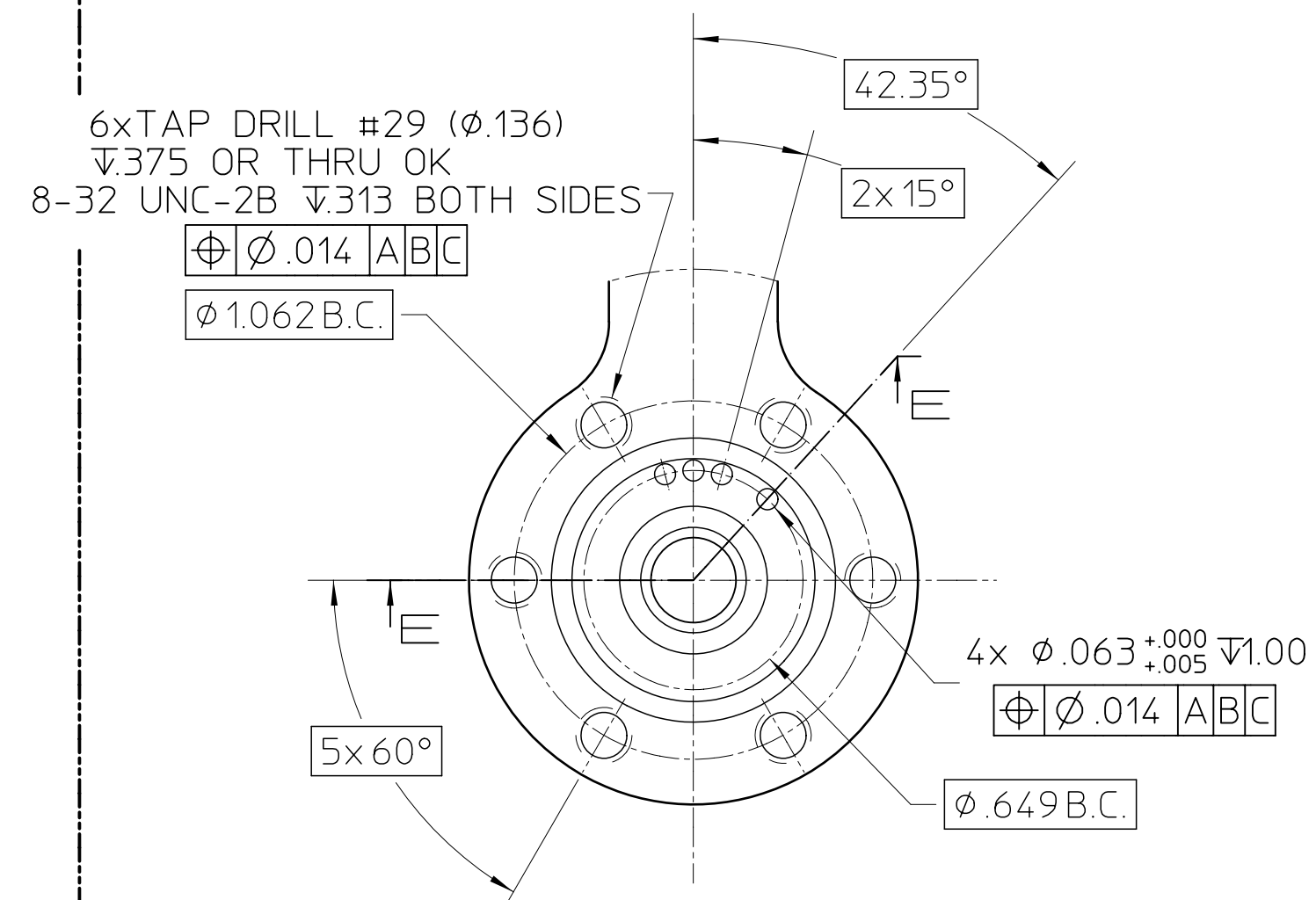
DETAIL 2 TYP BOTH SIDES SCALE 2/1 STANDARD 1-1/3 MINI-CFF KNIFE EDGE ROTATED 12° FOR CLARITY
