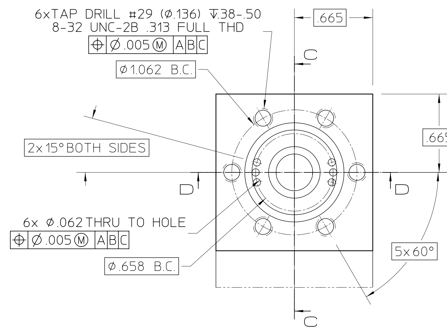
DETAIL 1 SCALE 2/1 STANDARD 1-1/3 MINI-CFF KNIFE EDGE
