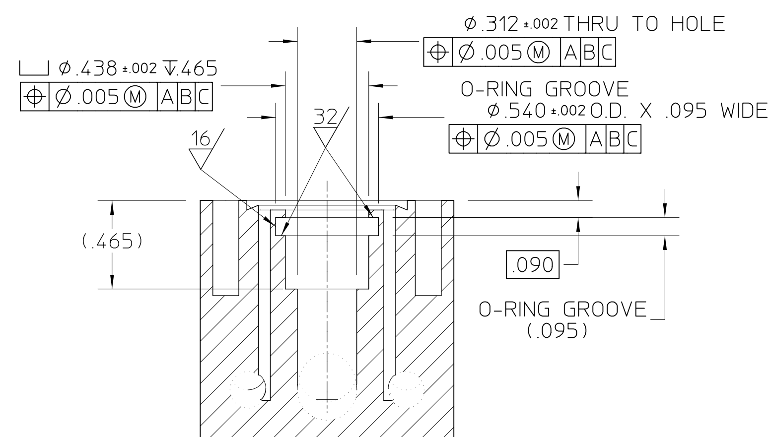
SECTION D-D SCALE 2/1 STANDARD 1-1/3 MINI-CFF KNIFE EDGE
