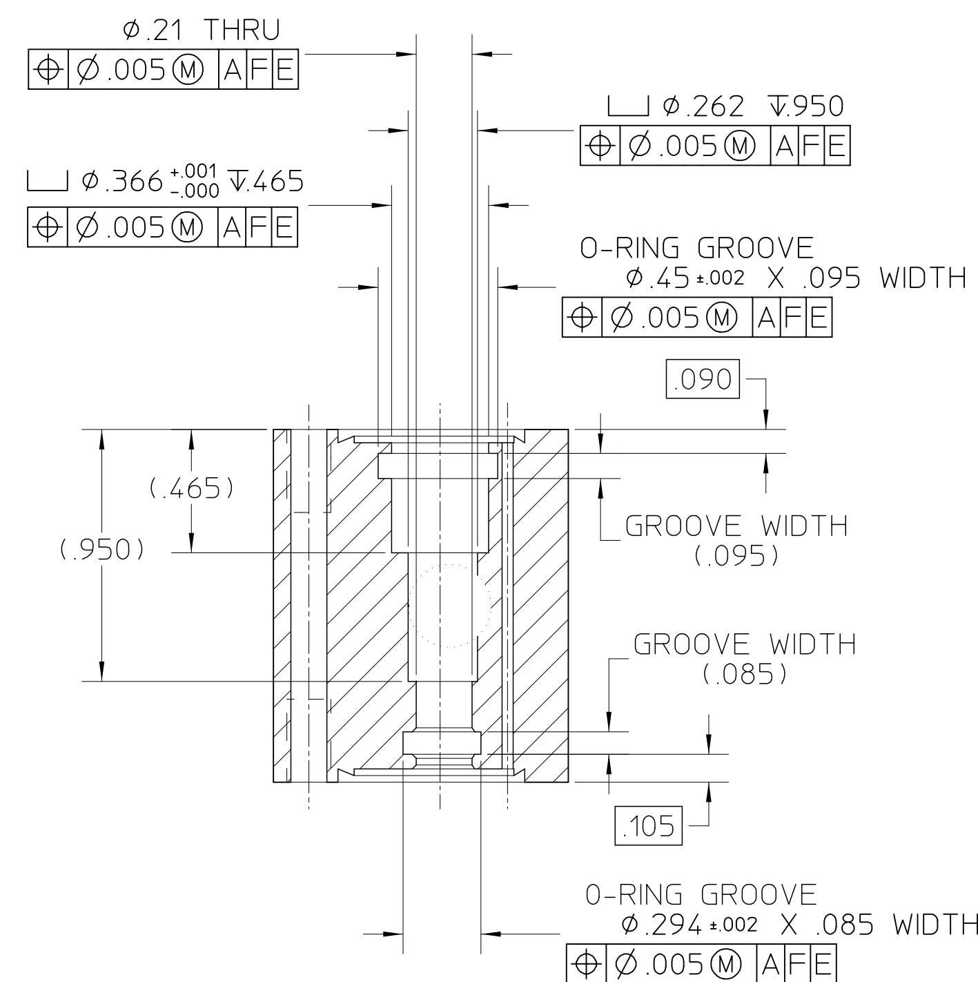
SECTION E-E SCALE 2/1 STANDARD 1-1/3 MINI-CFF KNIFE EDGE
