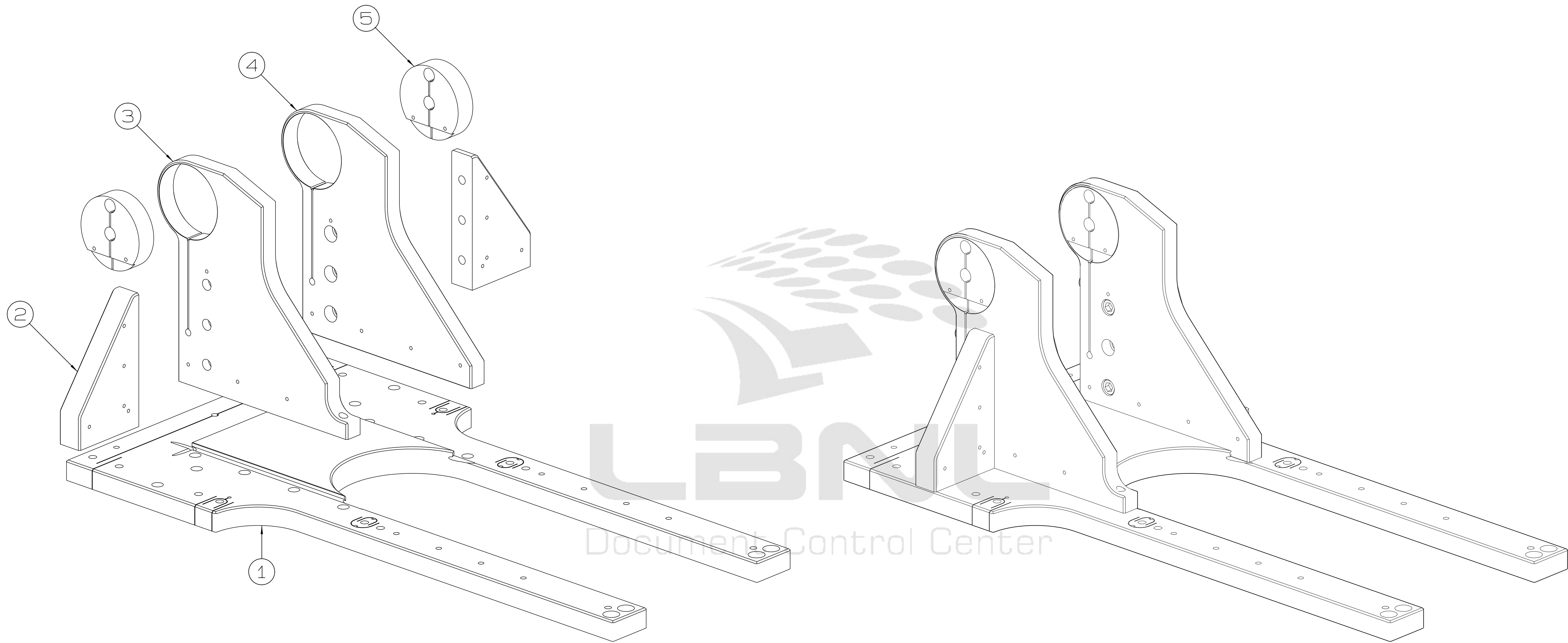
EXPLODED VIEW
