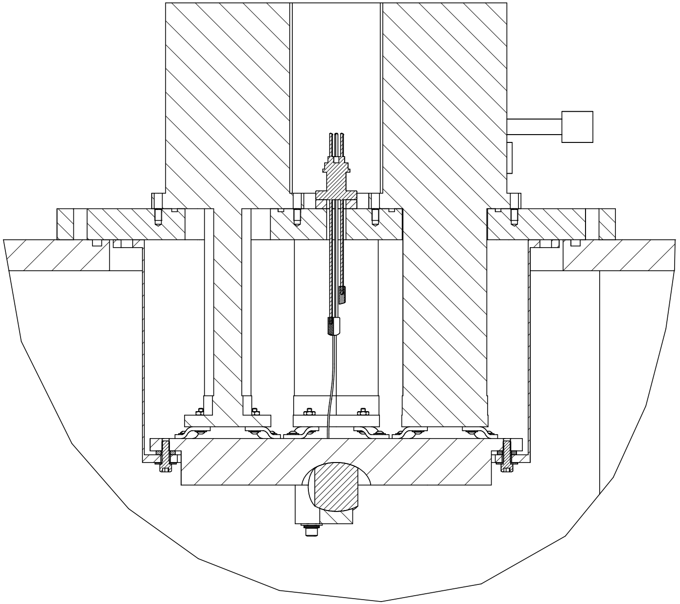
SECTION B-B SCALE 33/100
