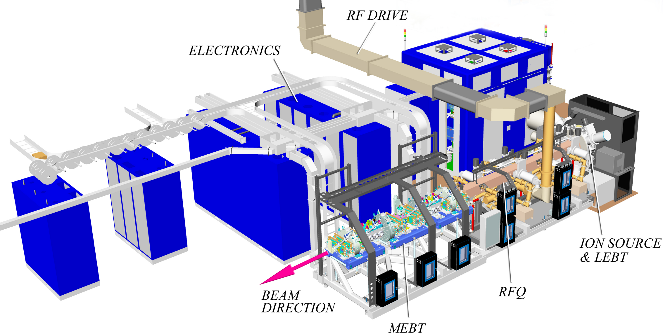
SNS - FRONT END SYSTEM
