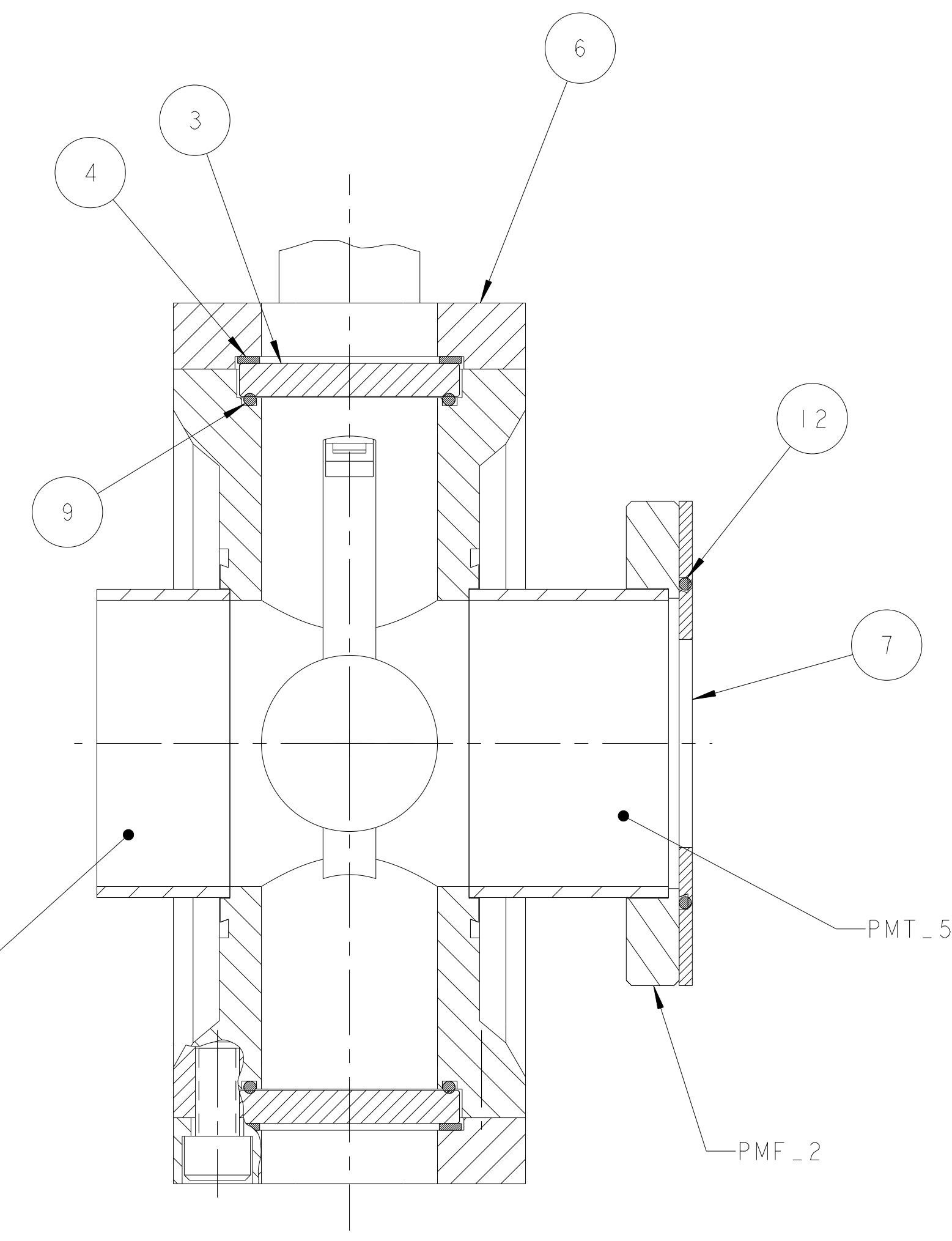
SECTION B-B SCALE 3/2
