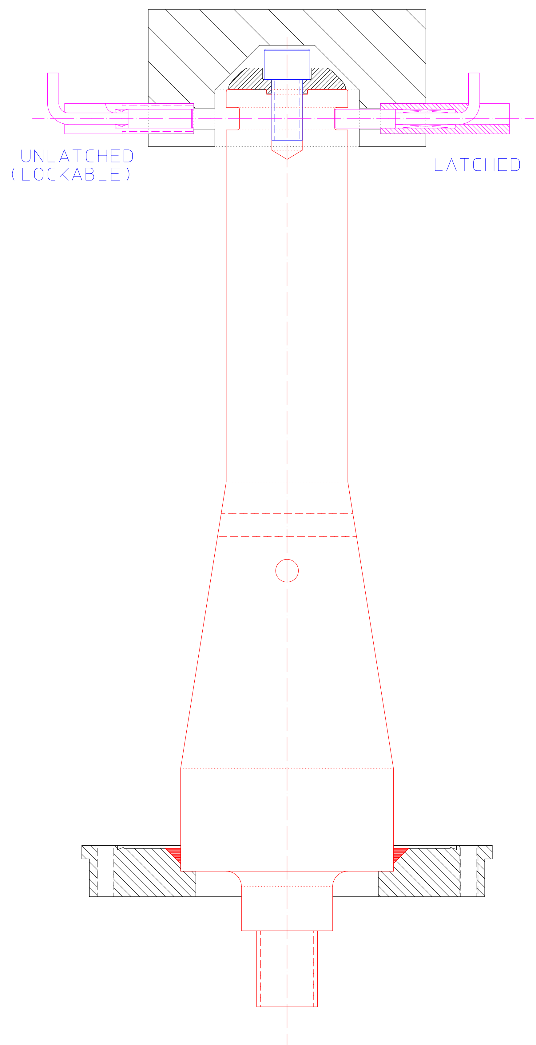
SECTION B-B
